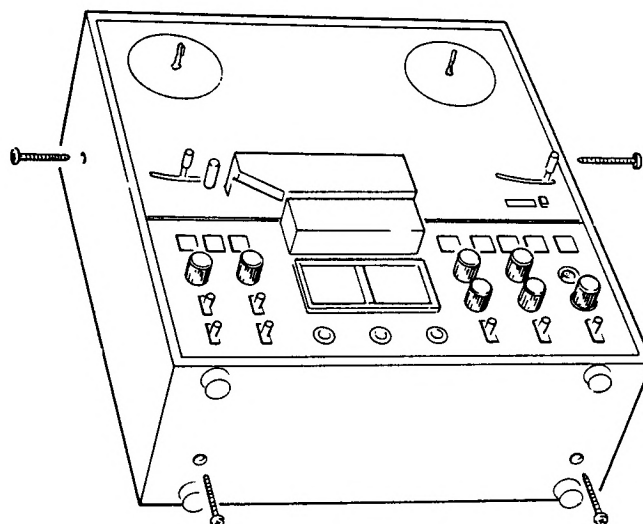
Cabinet screws
