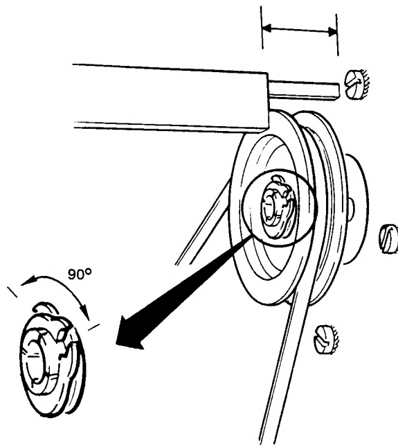
Motor pulley with circlips
