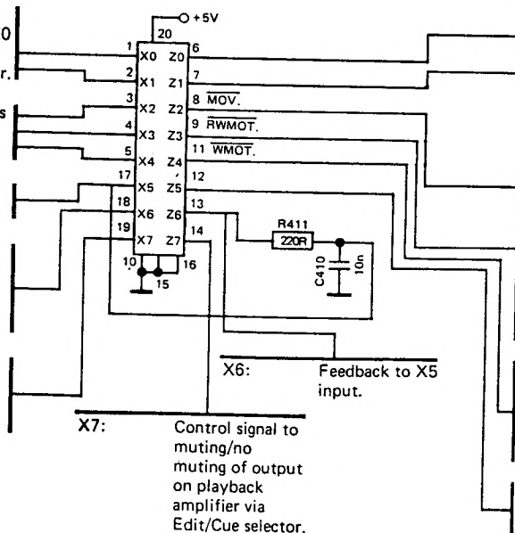
Inputs and Outputs on U3
