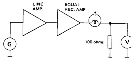
Checking the record curve
