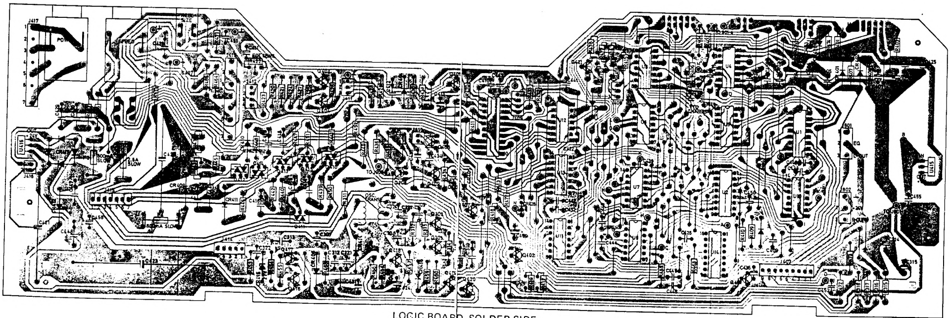
LOGIC BOARD, SOLDER SIDE
