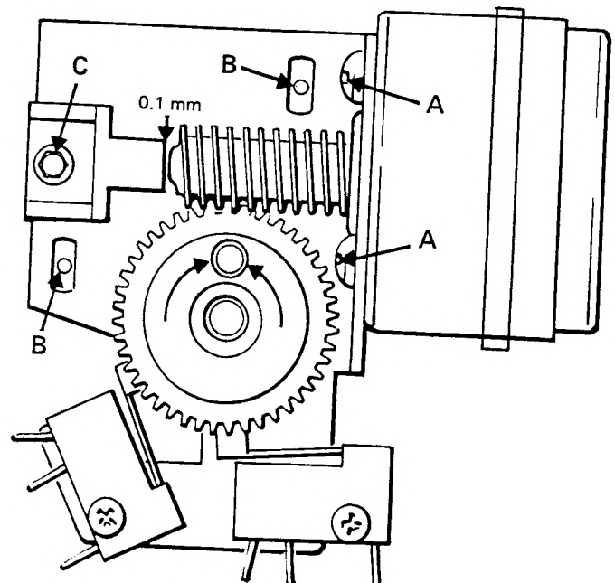
Adjusting the worm-gear motor
