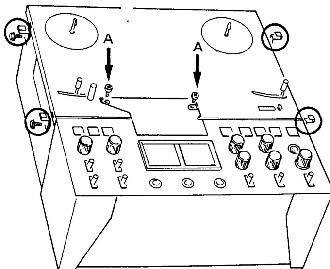
Removing and replacing the black top cover
