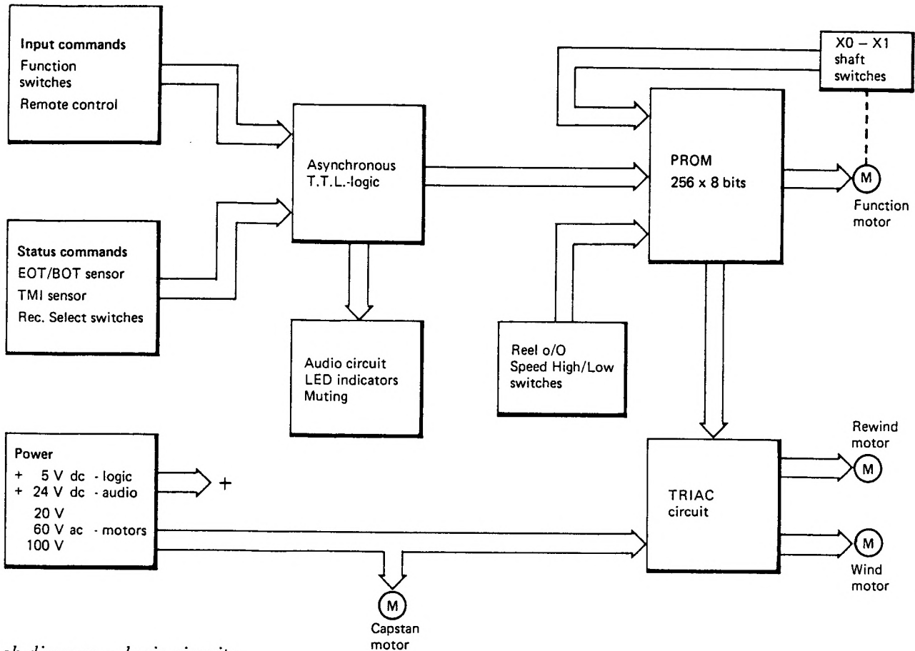
Block diagram – logic circuits
