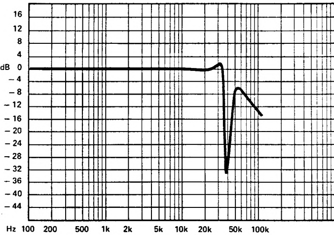
38 kHz trap curve
