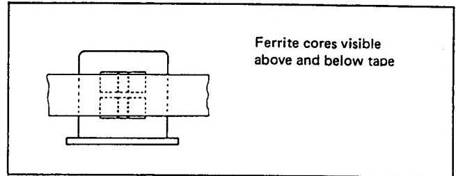
Two track erase head
