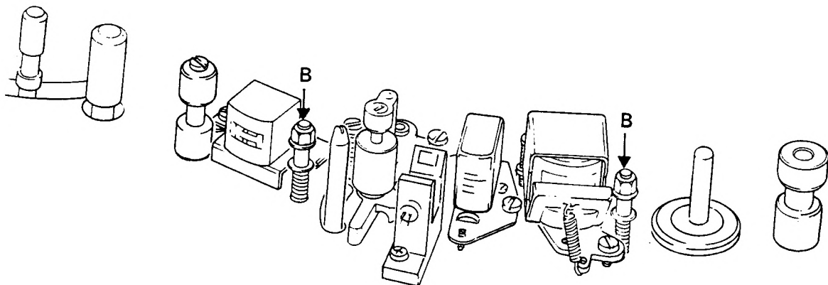
Adjustable tape guide posts
