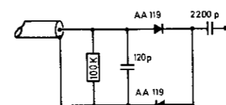
Figure 5 Diode probe
