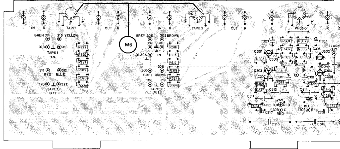
Seen from the solder side.
