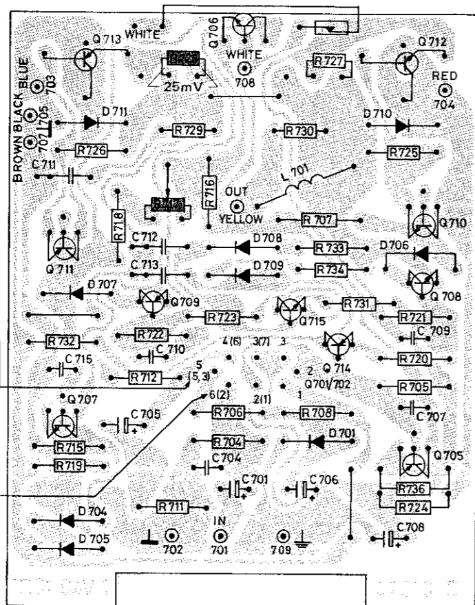
Seen from the solder side.
