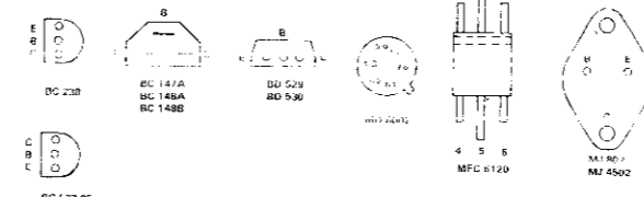
The transistors are seen from underneath (the lead or terminal side).
