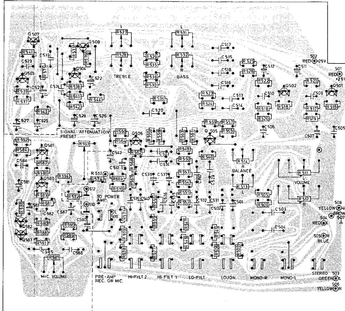
Seen from the solder side.
