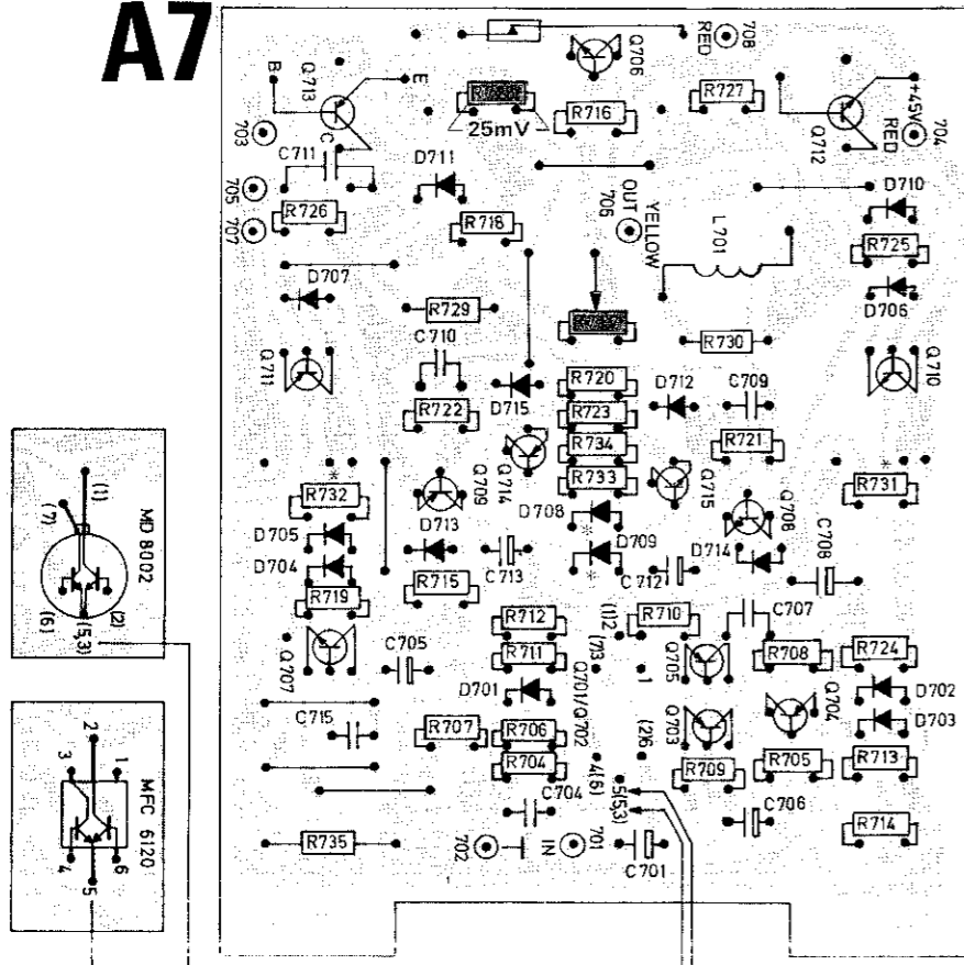
Seen from the solder side.
