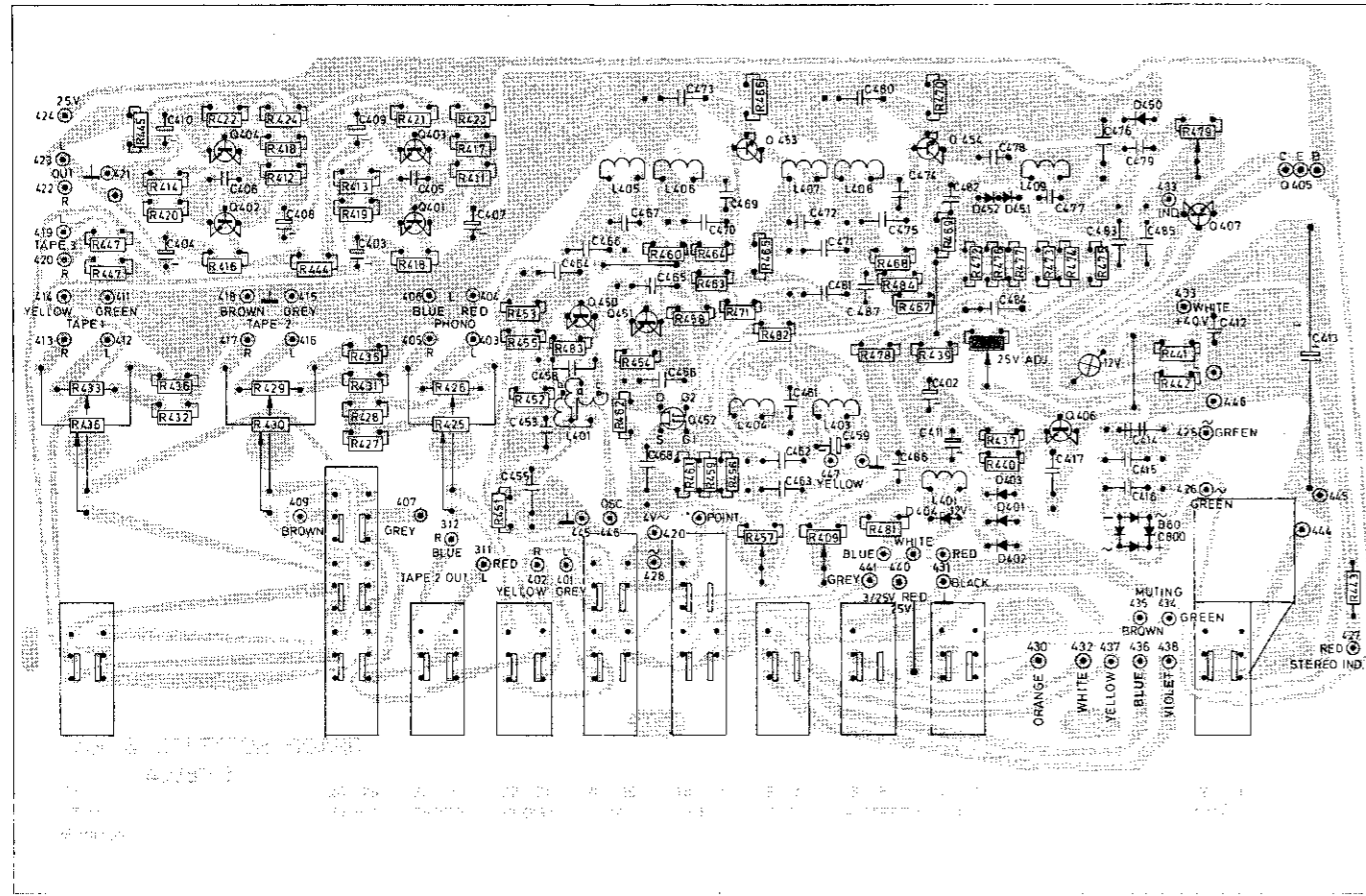
Seen from the solder side.
