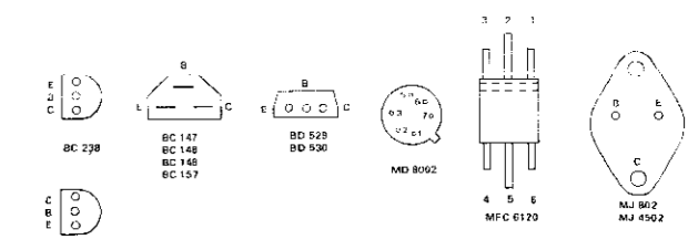
The transistors are seen from underneath
