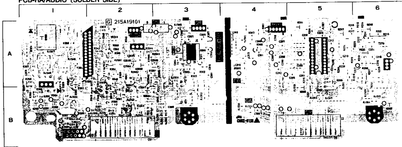
PCB-HA/AUDIO (SOLDER SIDE)
