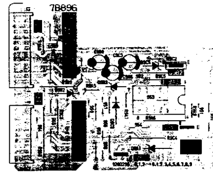
PCB-POWER-SUB 2 [COMPONENT SIDE]
