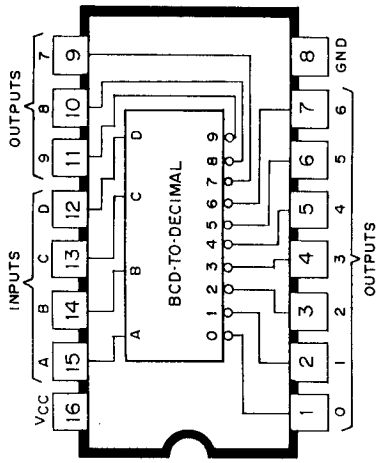
IC609: M74LS145
