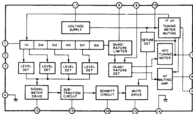
IC1: LA1235
