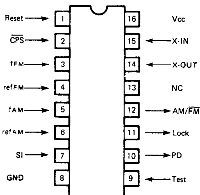
IC4: M54927P
