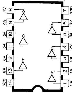
IC614: M74LS04
