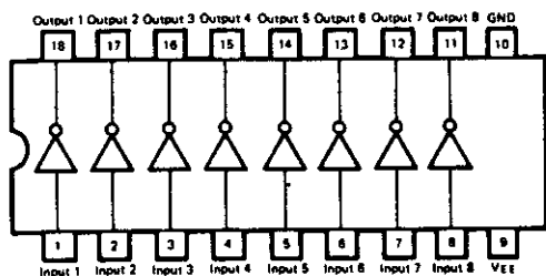
IC3: AN6873 (Indicator Circuit)
