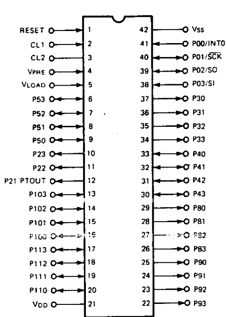
IC1(Tuner Circuit), IC607: \mu PD7538
