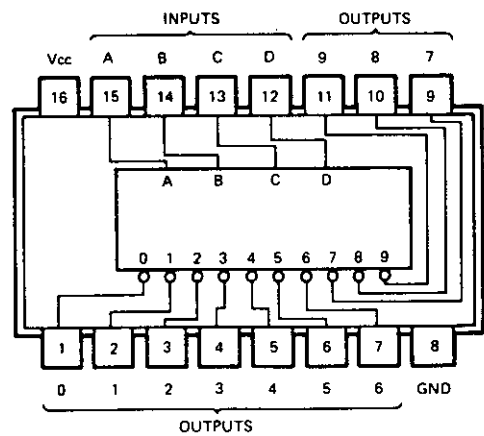
IC4: M74LS42 (Indicator Circuit)
