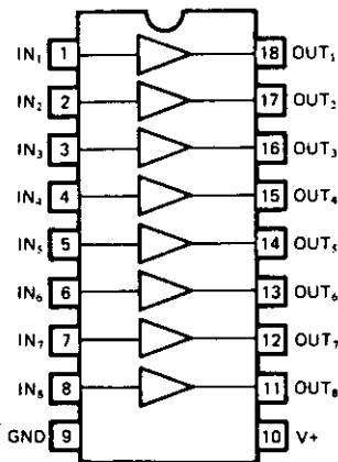
IC2: MSL912RS (Indicator Circuit)
