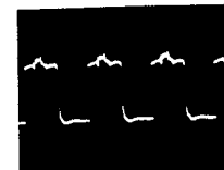
⑬0.7Vp-p(H)
