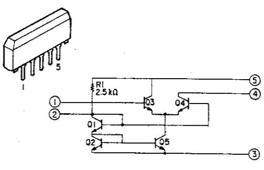
TA-7060AP
