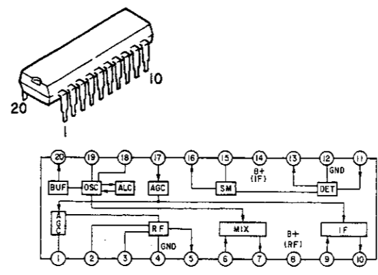
LA1247
