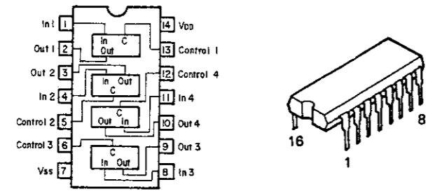
LM7001
