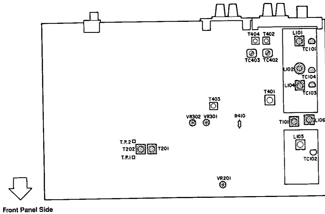
KU-9265 TUNER UNIT FM Alignment Points (Component Side)
