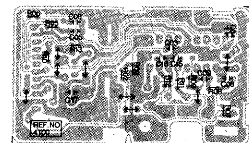
SOLDER SIDE
