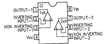
BA4558F (SU: IC101, 103, 261, 263) NJM2068MD (SU: IC101): Europe model only
