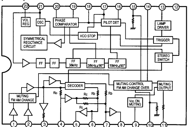
LA3401 (IC403)
