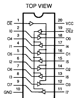
MM74LCX244 (IC818,819)
