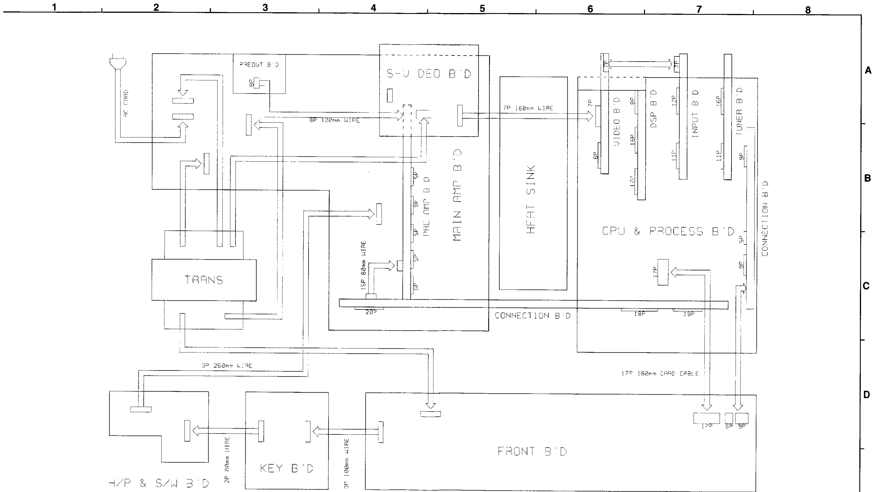
AVR1802 WIRING DIAGRAM
