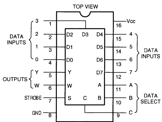
MM74HC151 (IC832)
