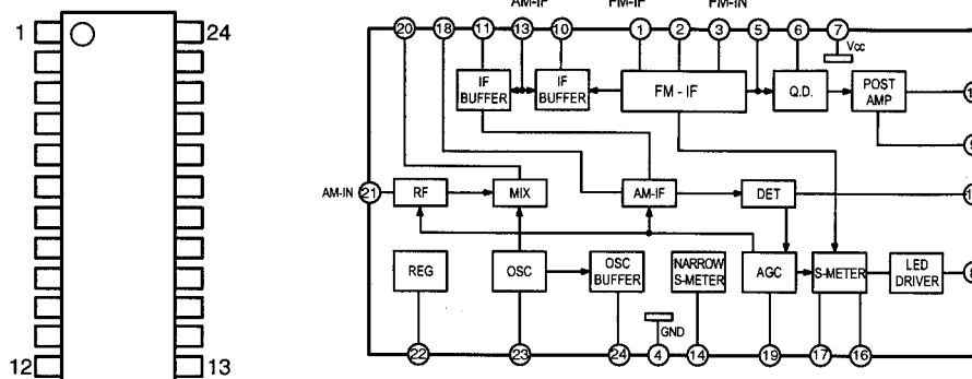
LA1266 (IC402)
