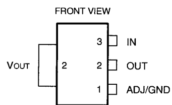
RC1117S25T (IC820) RC1117S33T (IC811)
