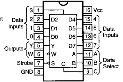
TC74HC151AF
