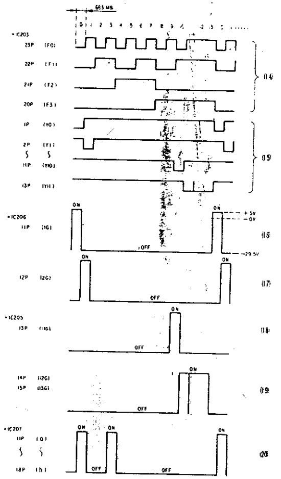
Oscilloscope 1 ms/div
