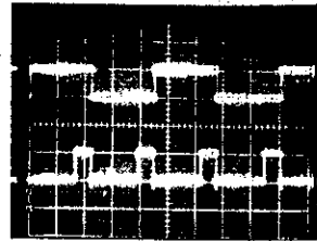
5 μsec/DIV, 5V/sec
