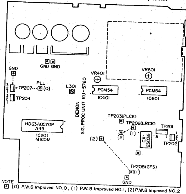
Signal Processing PWB Location of Terminal for Adjustment
