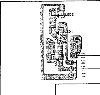
61F LED
