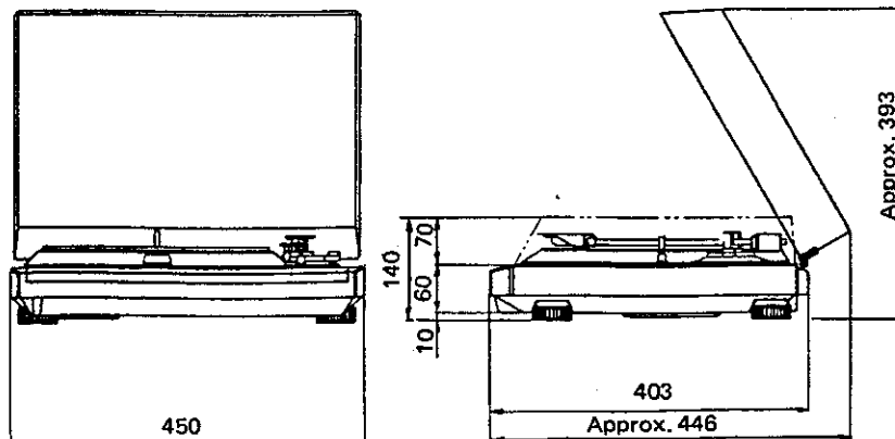
Dimensions (mm)
