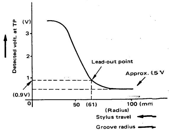
Fig. 9 Voltage Transition vs Stylus Travel
