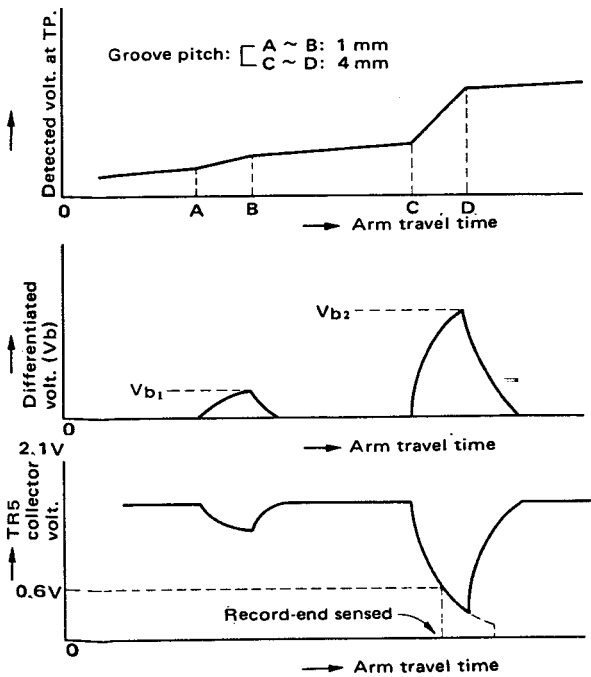
Fig. 10 Differentiated Voltage
