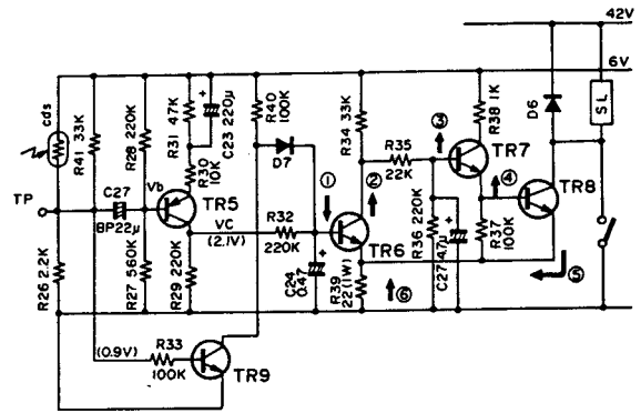
Fig. 11 Detection Circuit
