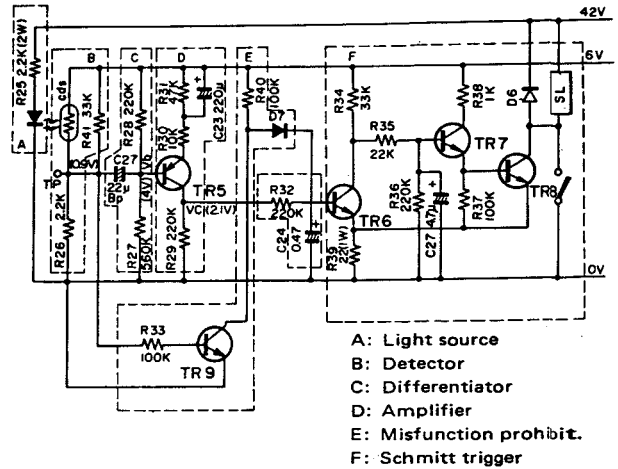
Fig. 8 Detection Circuit
