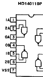
HD14011BP HD14066BP HD14082BP (Hitachi)
