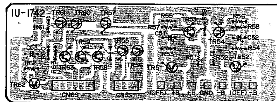
1U-1742 CONTROL UNIT (DRA-625R/425R)
