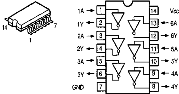
TC74HC04AF (IC103)
