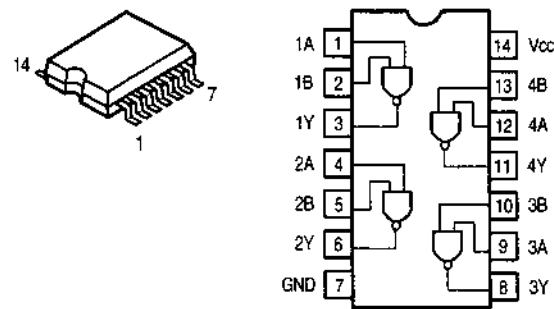
TC74HC004AF (IC104)
