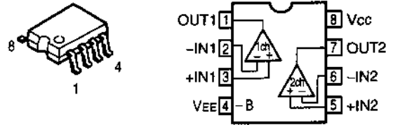
NJM4565MD (IC 101,102, 110)
