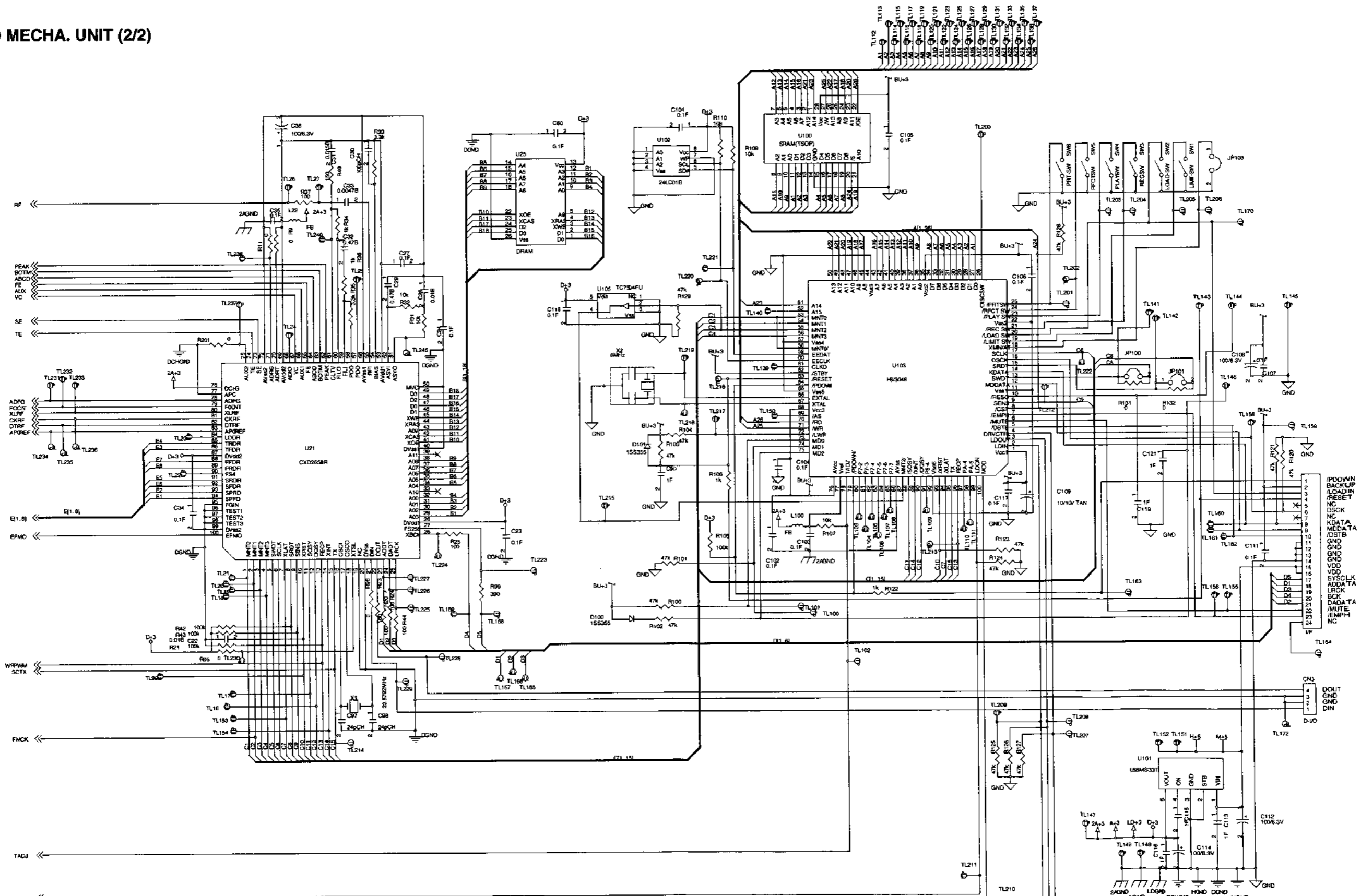
SCHEMATIC DIAGRAMS (3/3) MD MECHA. UNIT (2/2)
