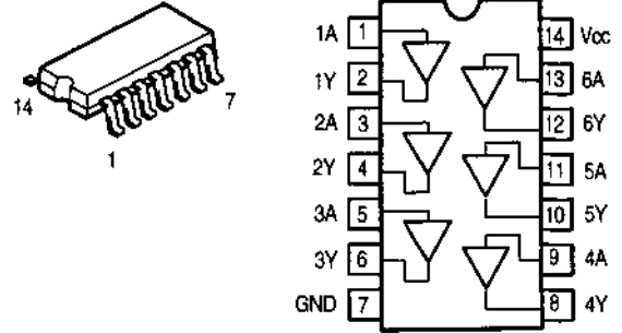
TC74HC7007AF (IC105,112)
