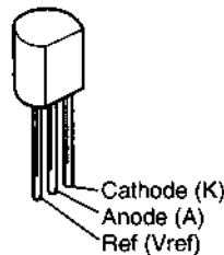
TL431CLP (IC113)
