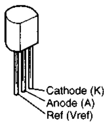
TL431CLP (IC113)
