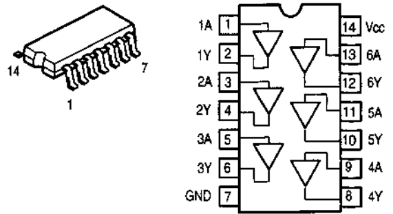
TC74HC7007AF (IC105,112)
