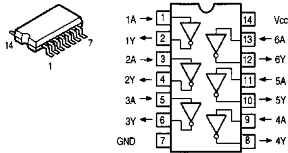
TC74HC04AF (IC103)
