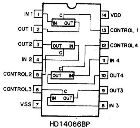
HD14066BP
