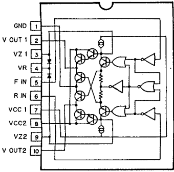
BA6109
