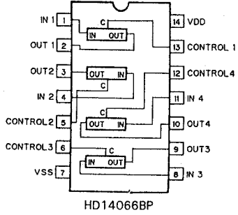
HD14066BP
