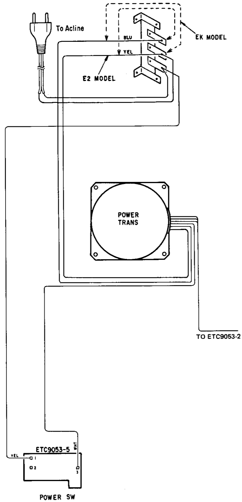
WIRING DIAGRAM E2 & EK Models (Same as EU version except the following)
