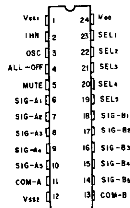
TC9152P (Toshiba)
