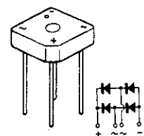
RB402ULF-F
