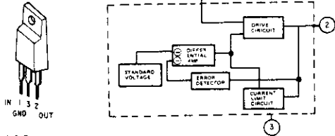
μPC741C
