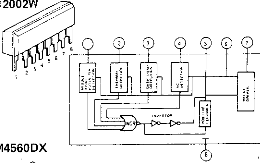
HA12002W
