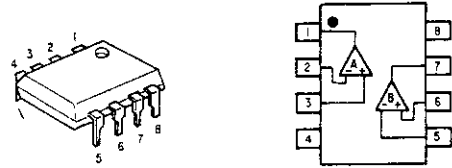
NJM082D
