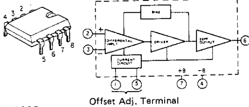
NJM082D
