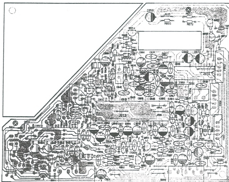
PT2 NICAM L BOARD / PT2 NICAM L BAUSTEIN / CIRCUIT IMPRIME DU PT2 NICAM L
