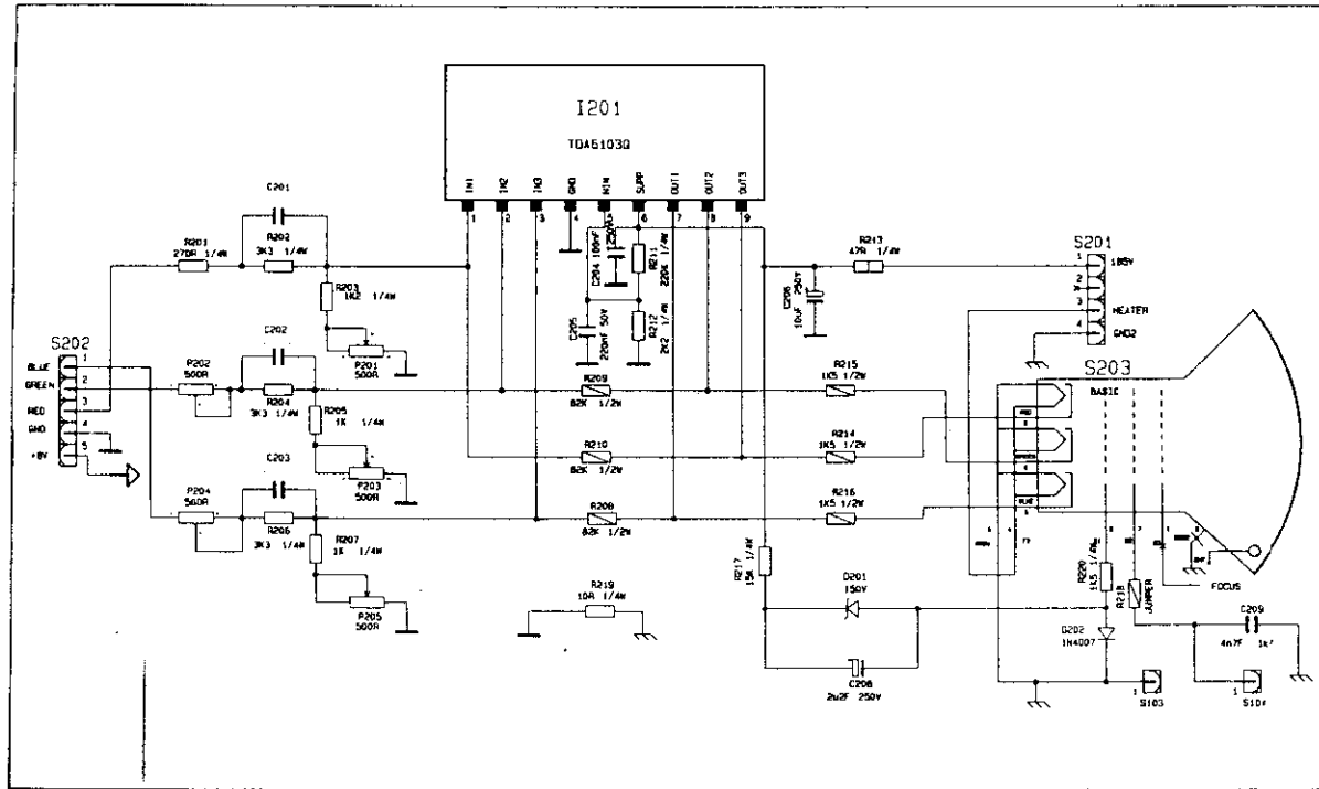
TDA 6103 CRT BOARD CIRCUIT DIAGRAM / TDA 6103 CRT BAUSTEIN SCHALTUNGSPLAN / SCHEMA DU CIRCUIT TDA 6103
