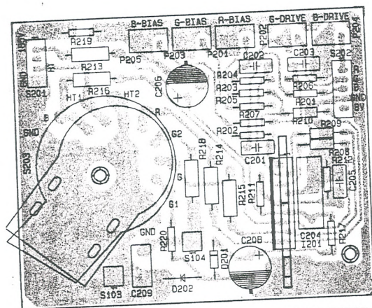
TDA 6103 CRT BOARD / TDA 6103 CRT BAUSTEIN / CIRCUIT IMPRIME DU CRT TDA 6103
