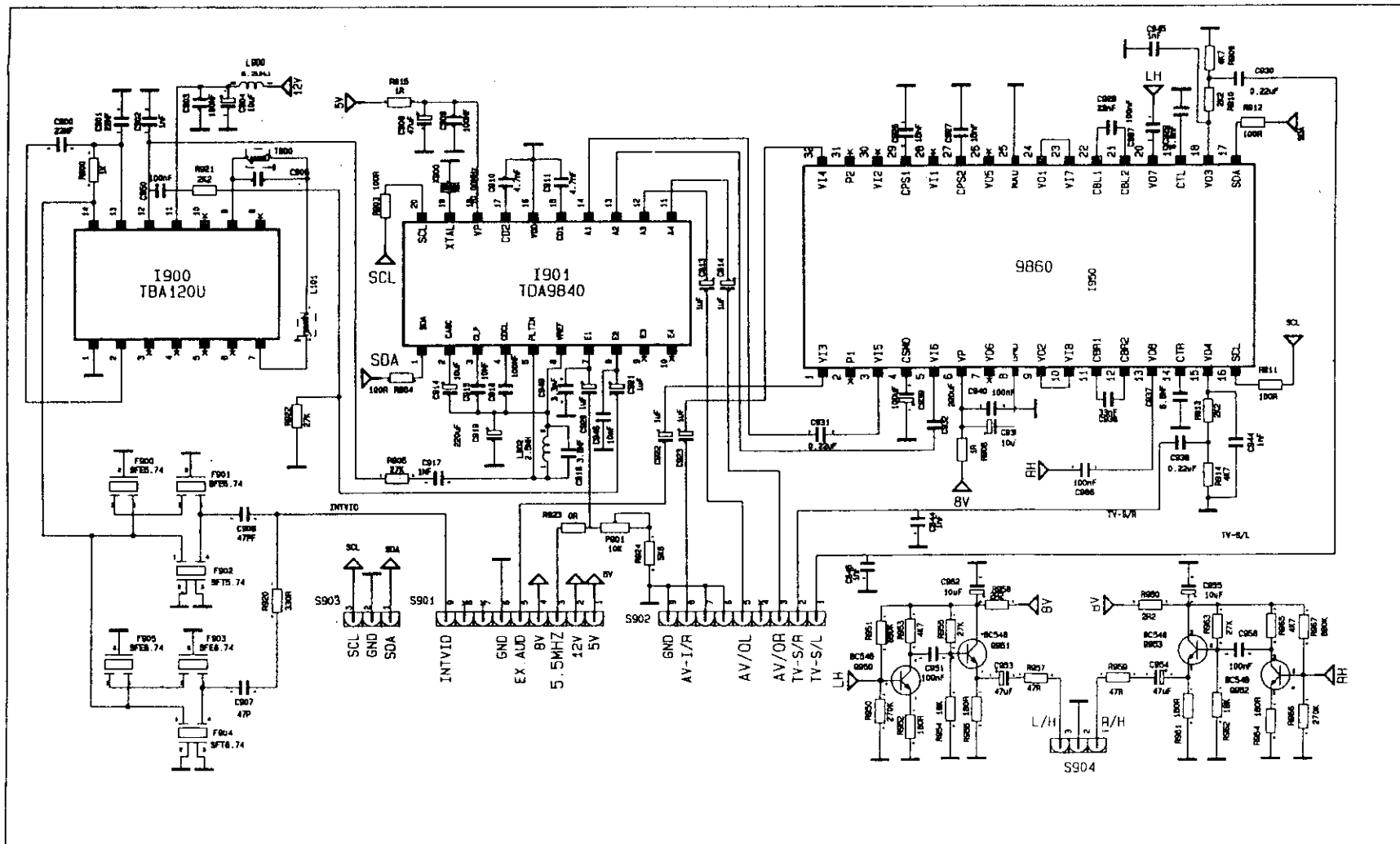
PT2 GERMAN STEREO BOARD CIRCUIT DIAGRAM / PT2 GERMAN STEREO BAUSTEINSCHALTUNGSPLAN / SCHEMA DU CIRCUIT GERMAN STEREO
