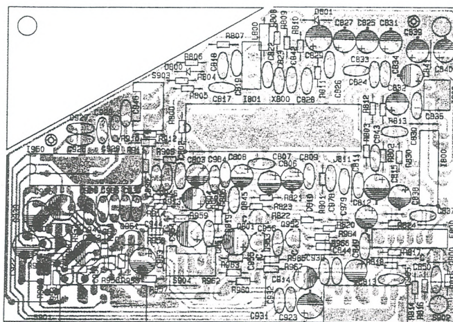
PT2 NICAM STEREO BOARD / PT2 NICAM STEREO BAUSTEIN / CIRCUIT IMPRIME DU PT2 NICAM STEREO
