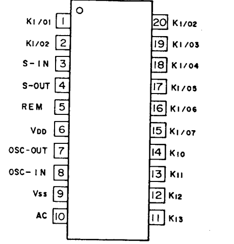
IC μPD6600GD-519 Pin Connection Diagram (Top View)
