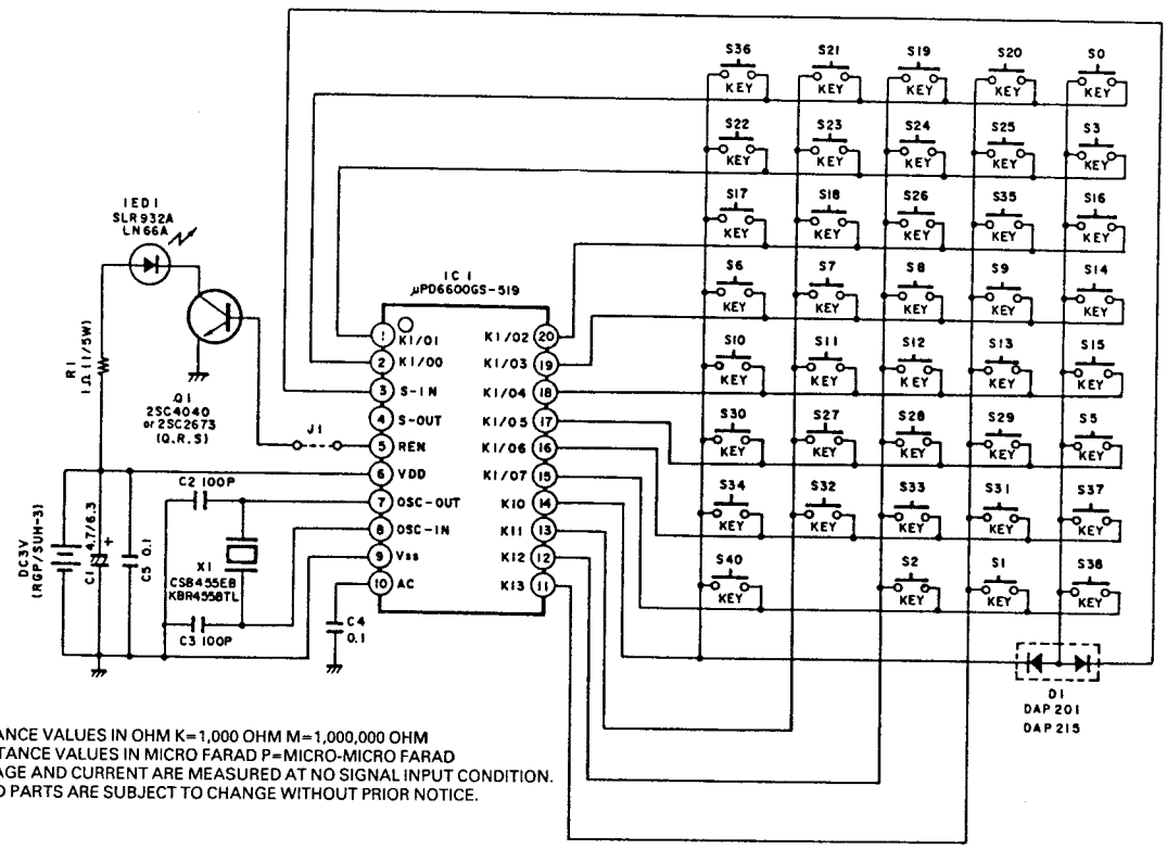
Schematic Diagram
