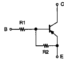
PNP Type
