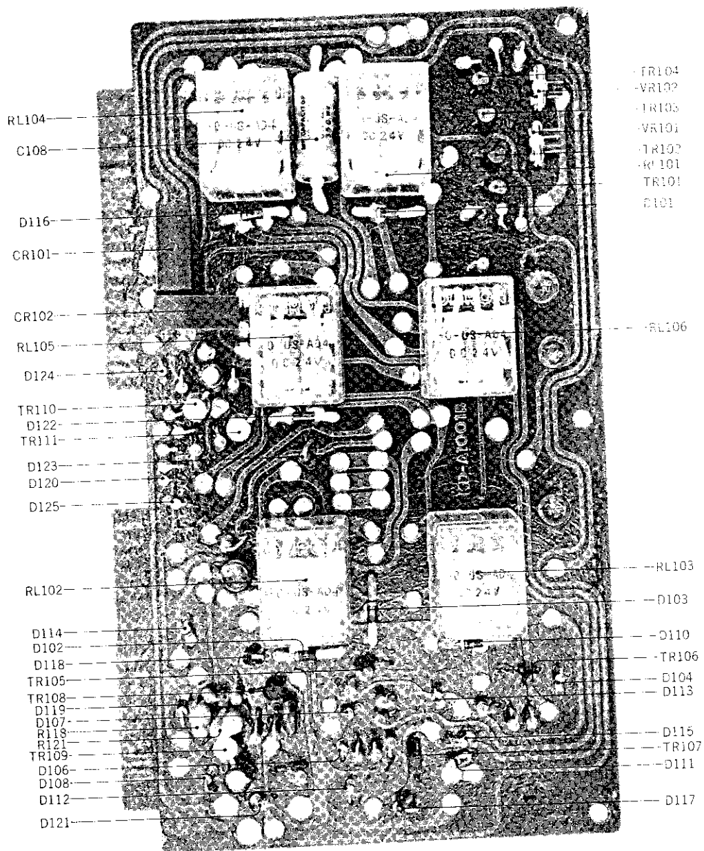
FIG. 10 PHOTO OF SYS. CON. P.C. BOARD (KD-A1001A)
