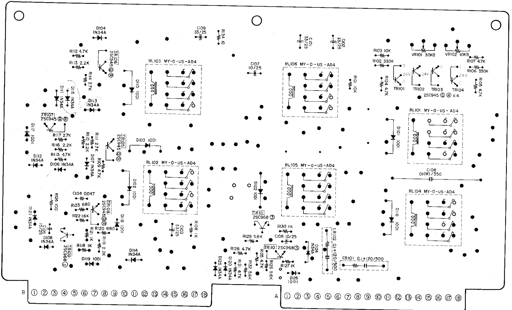
Fig. 26 SYSTEM CONTROL P.C. BOARD KD-A1001 (Reverse Side)
