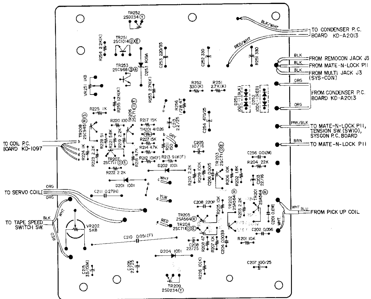
Fig. 32 SERVO CONTROL AMP. & POWER SUPPLY P.C. BOARD KD-1096 (Reverse Side)
