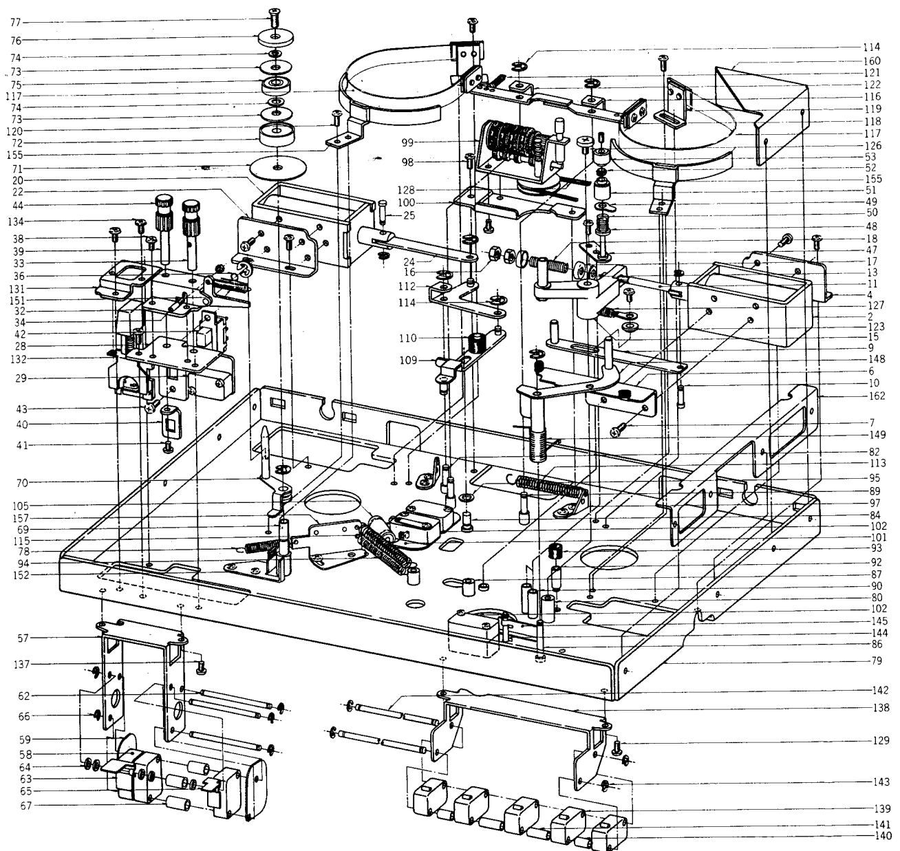
FIG. 5 ILLUSTRATION OF MECHANISM ASSEMBLY BLOCK (1)
