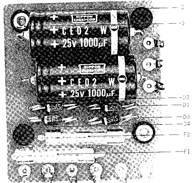
FIG. 18 PHOTO OF POWER SUPPLY P.C. BOARD (KD-A5020)
