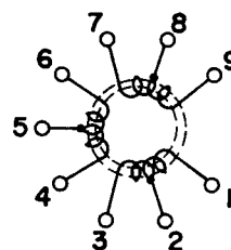
OSCILLATOR COIL
