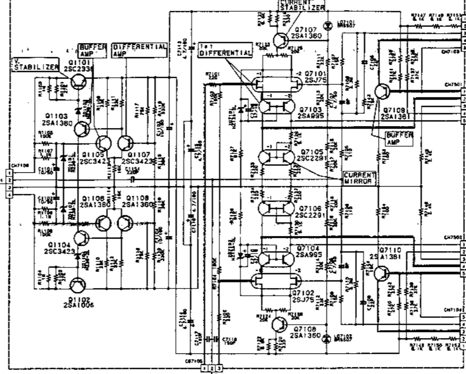
DRIVER P. C. Board
