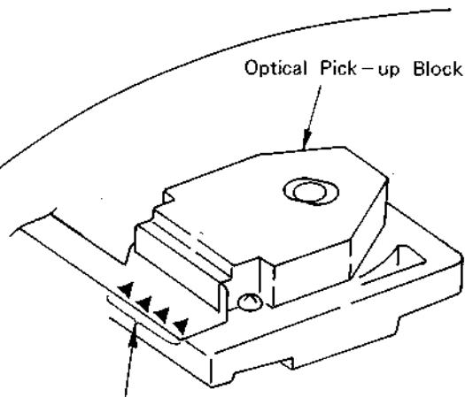
(2) Remove four solders "▲".
