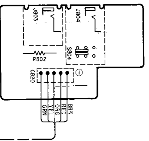
Remote P.C. Board
