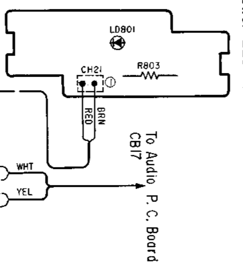
Power LED P.C. Board
