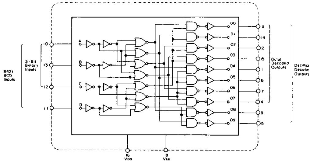
MC14028BCP: (Stock No. 51T51782F01)
