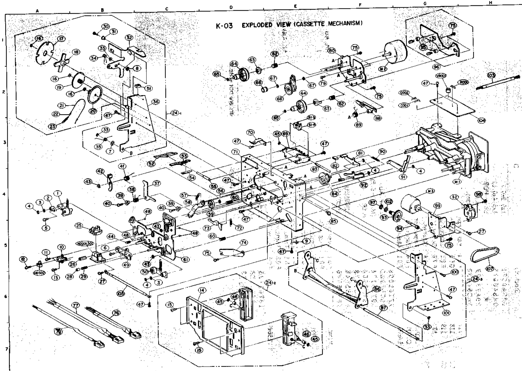
Exploded View (Mechanism)
