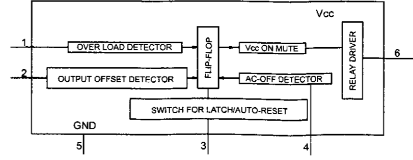
IC44: uPC1237HA
