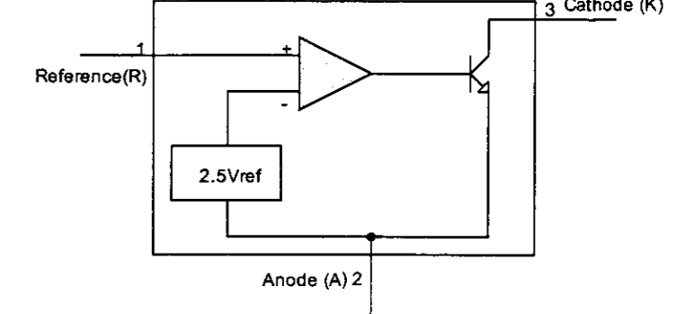
IC11, IC12, IC21, IC22: TL431
