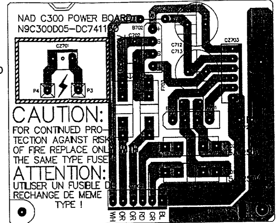
POWER BOARD
