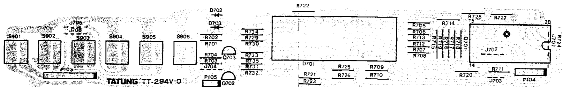
Display, PCB Layout
