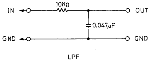
LPF
