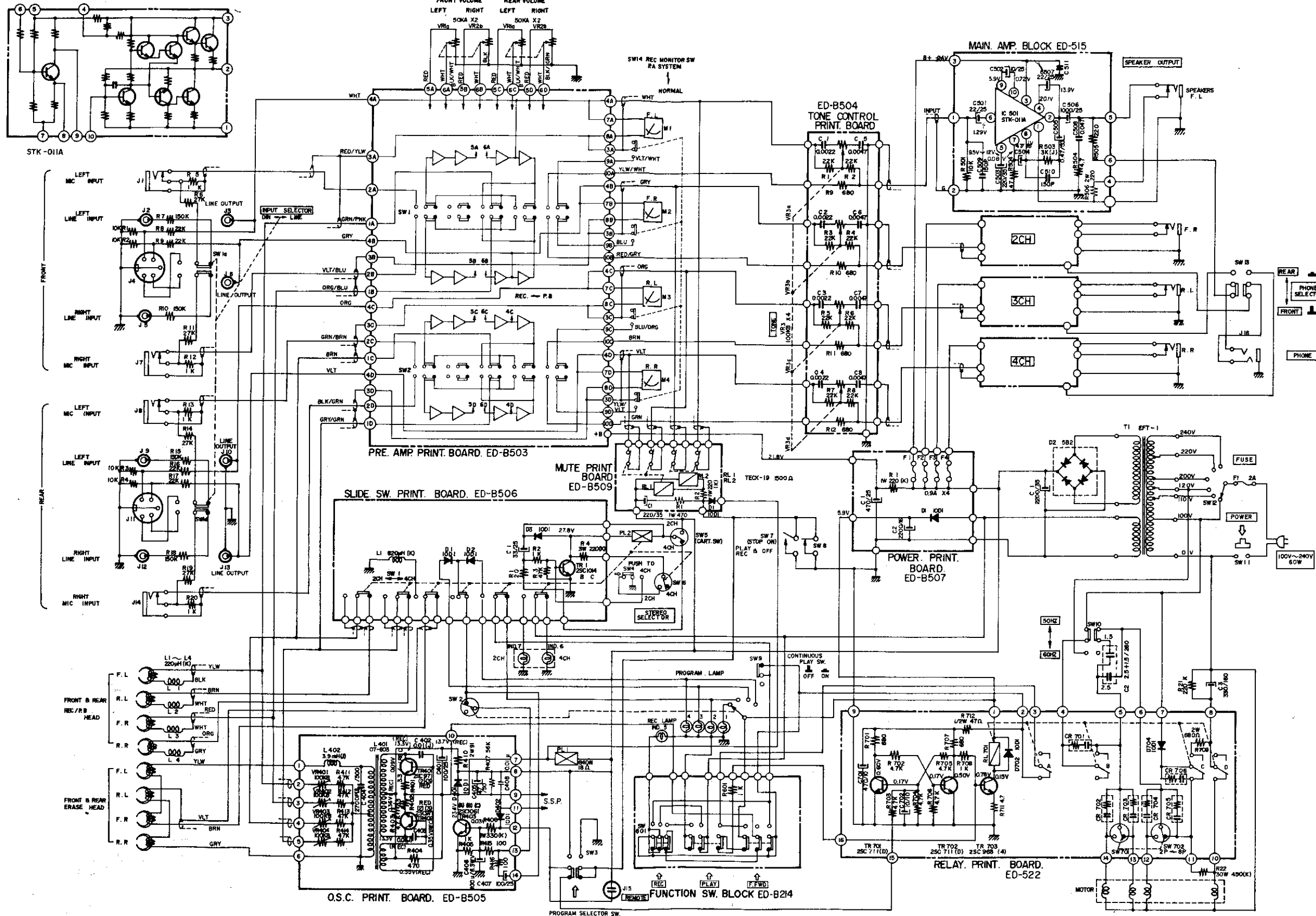
CR-80-SS MECHANISM SCHEMATIC DIAGRAM 1422050A
