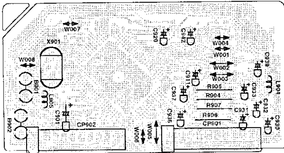
STEREO (INSERTED PARTS) SOLDER SIDE
