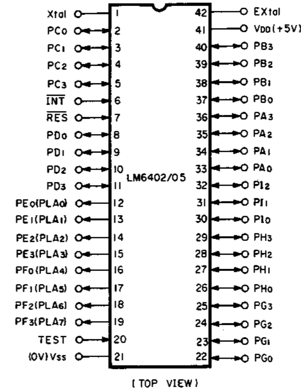
Fig. 13.12 4-Bit Micro-processor LM6402A-052/048
