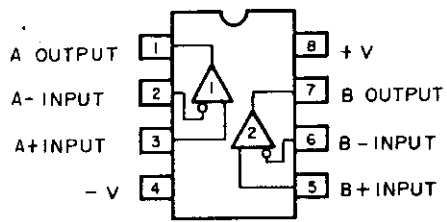
Operational Amp. IC M5220L, NJM4560D, BA4558 M5218L
