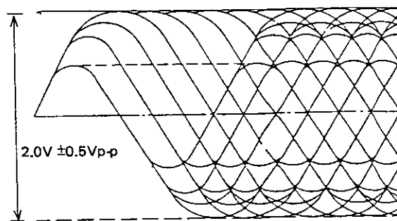
Fig. 3.9 EFM Signal
