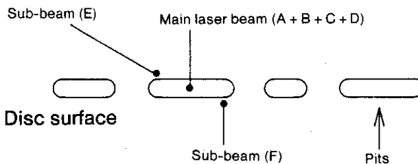
The 3-beam tracking servo
