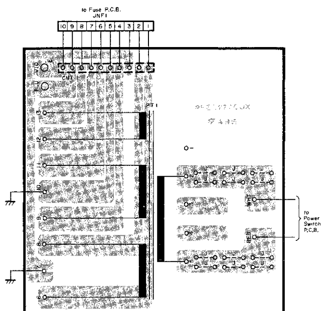
7.9. Power Transformer P.C.B. Ass'y
