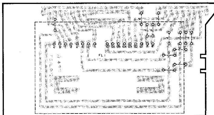
7.9. Power Transformer P.C.B. Ass'y
