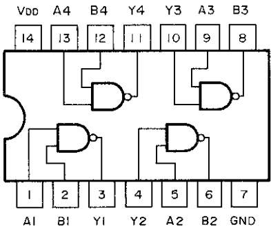
Fig. 8.1.2. NAND Gate C-MOS IC MN4011BP
