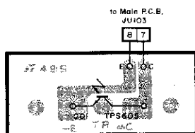
7.1. Photo Transistor P.C.B. Ass'y
