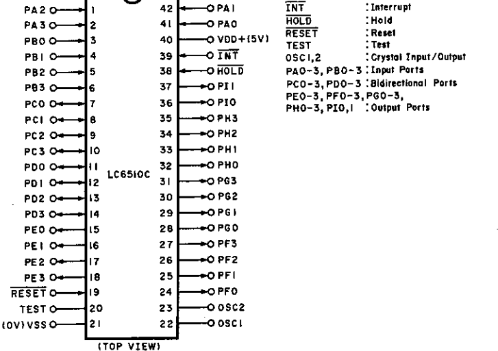
Fig. 8.1.14 4-Bit Micro-processor LC6510C-780
