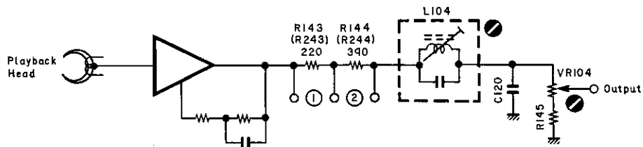
Fig. 5.4 Playback Amp.
