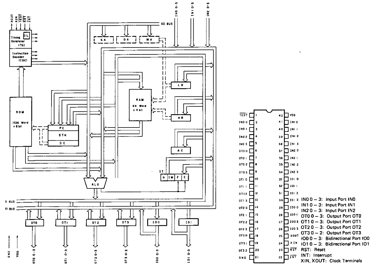
Fig. 8.1.11 4-Bit Micro-processor TMP4315BP-1814
