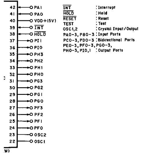
4-bit Micro-processor LC6510C-780
