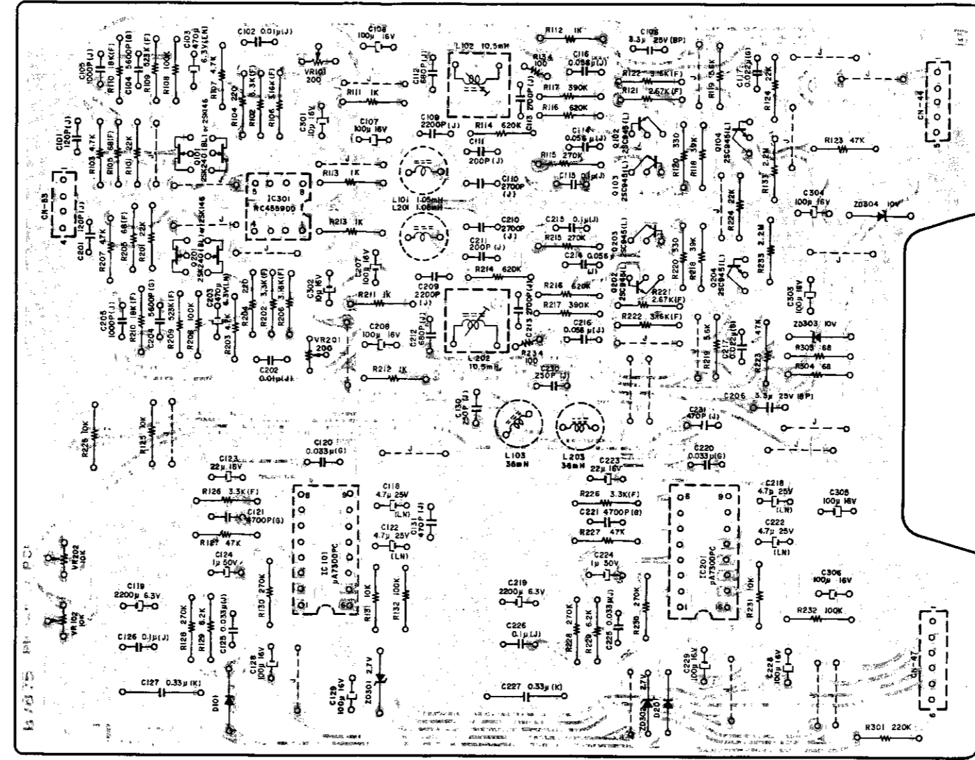
Fig. 1.17 Note: Diode is 1SS53 unless otherwise specified.
