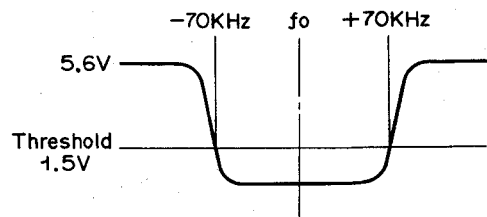
Fig. 2.4.13 Mute Out Signal
