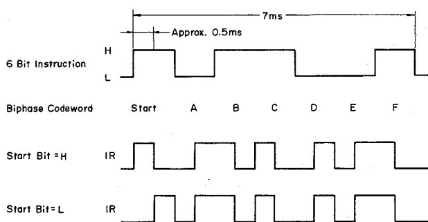
Fig. 2.6.2 Information Unit
