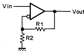
Fig. 2.1.14 Non-inverting
