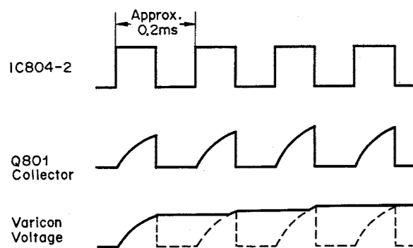
Fig. 2.4.6 Timing Chart
