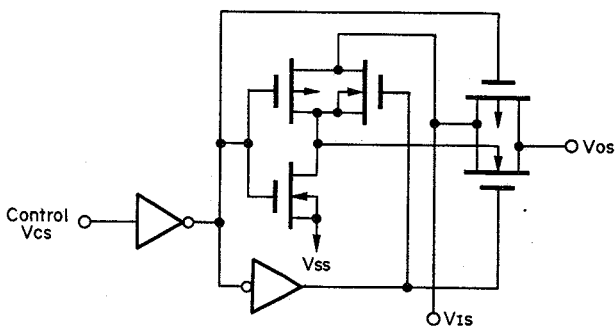
Fig. 2.1.11 Bilateral Switch
