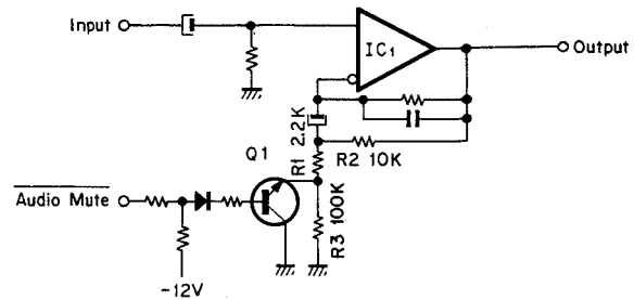
Fig. 2.5.5 Tone Control
