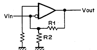
Fig. 2.1.15 Inverting
