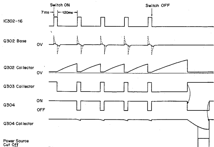
Fig. 2.6.5 Timing Chart
