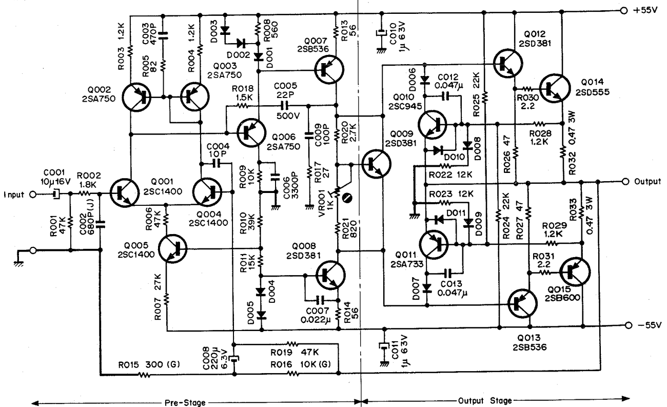
Fig. 2.5.8 Power Amplifier
