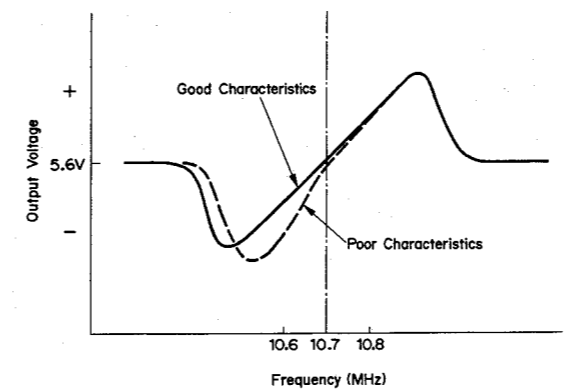
Fig. 2.4.4 Discriminator Characteristics (S-Curve)
