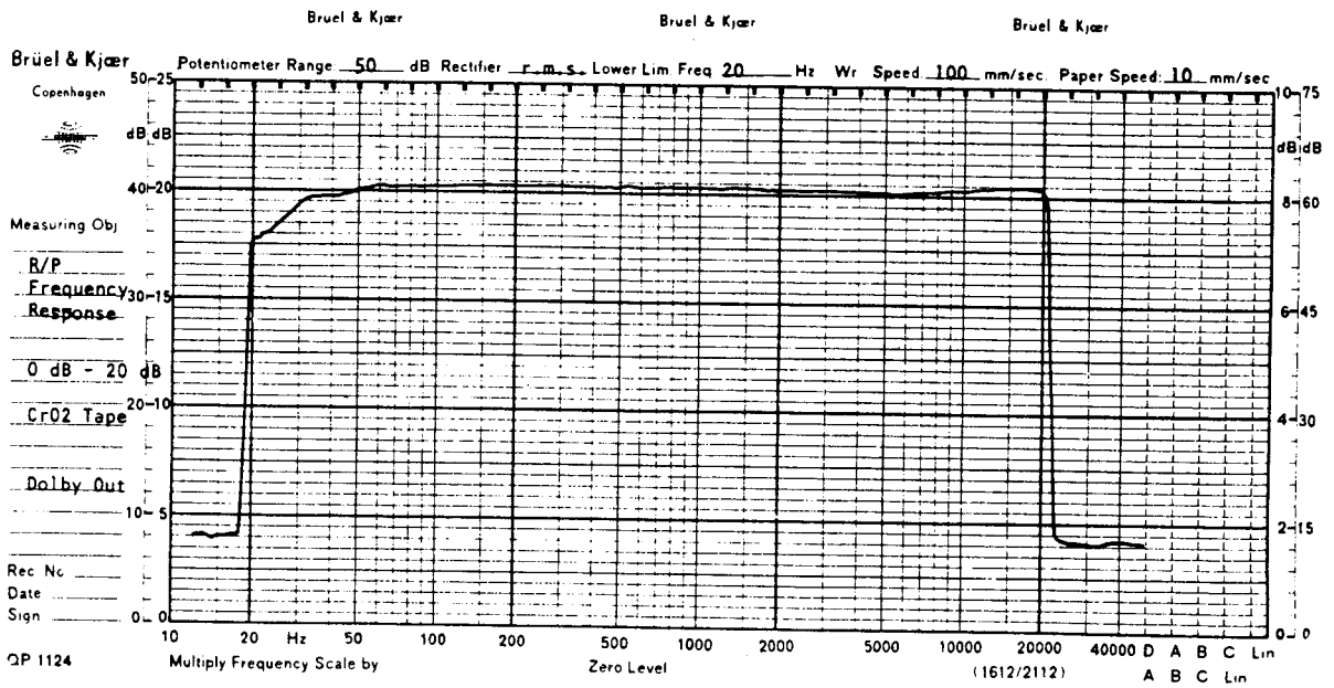
Fig. 2.19 Record/Playback Frequency Response (Dolby NR Out)
