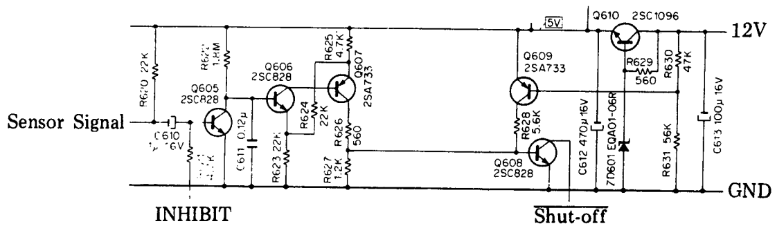
Fig. 2.26 Shut-off Sensor and Detector Circuit Diagram
