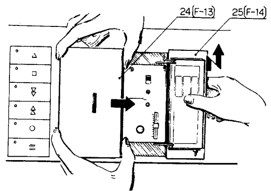
Fig. 3.1 Removal of Cassette Well and Lid
