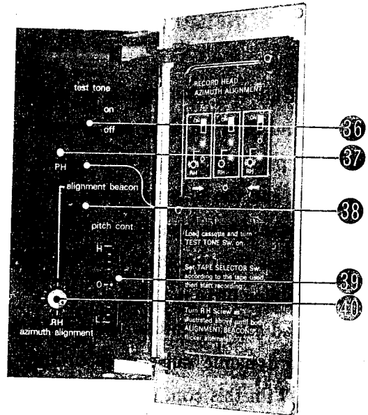
Fig. 1.3. (Adjustment Panel)
