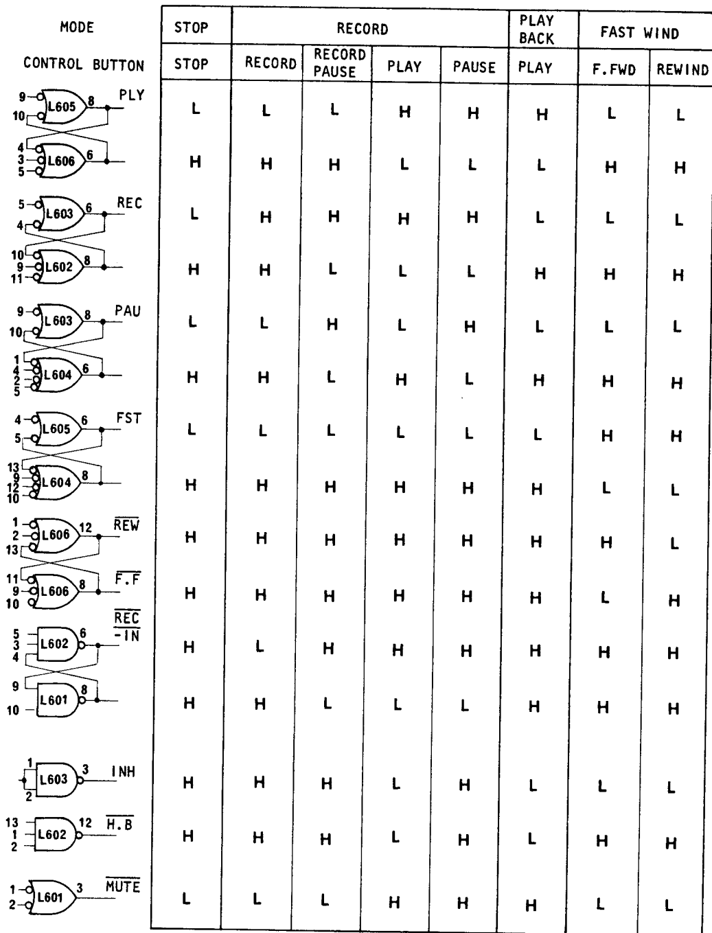
Fig. 2.25 Logic Status
