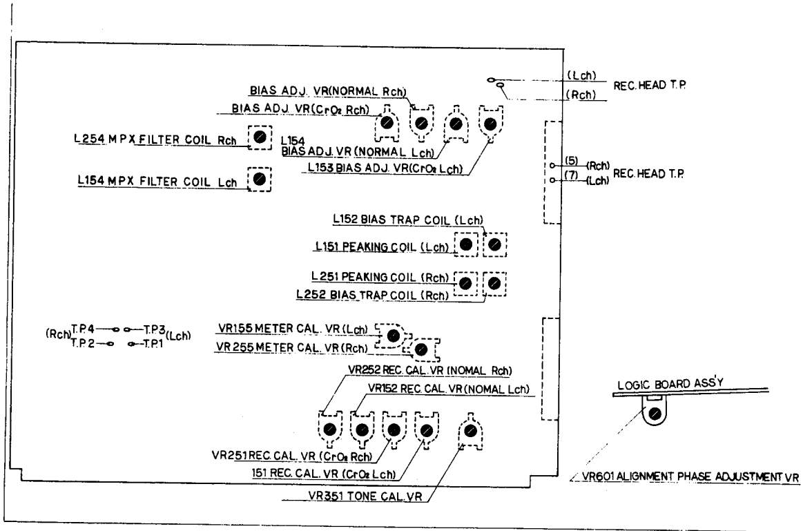
REAR VIEW
