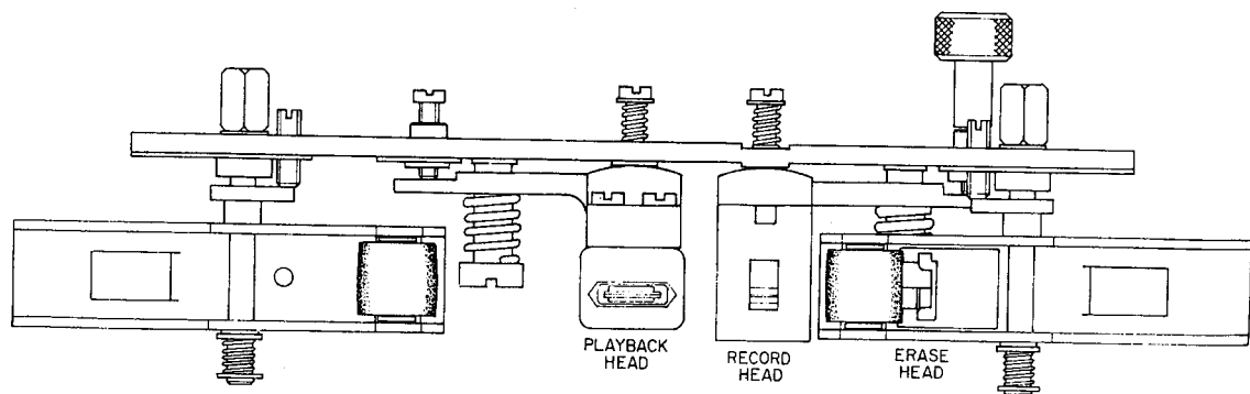
Fig. 2.1 Head Housing
