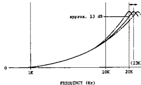
Fig. 6.22 Record Peaking Curve (1-7/8 ips)
