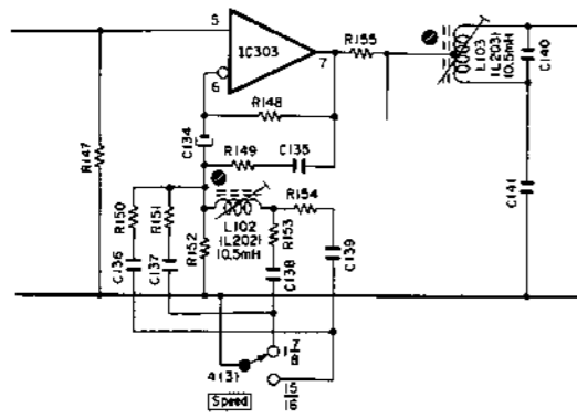
Fig. 6.6 10. Bias Oscillation Frequency and Erase Current
