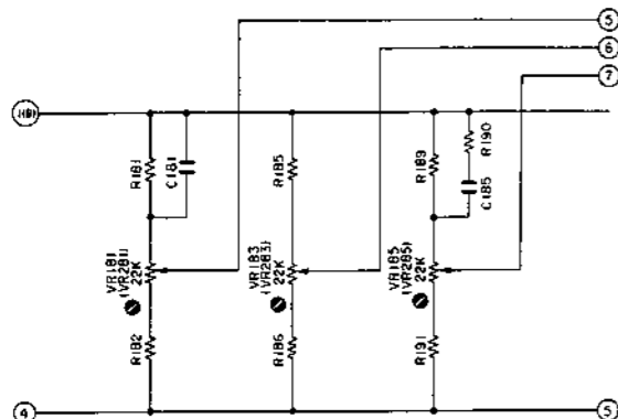
Fig. 6.14 15. Record Head Azimuth Phase 16. Record Level and Bias
