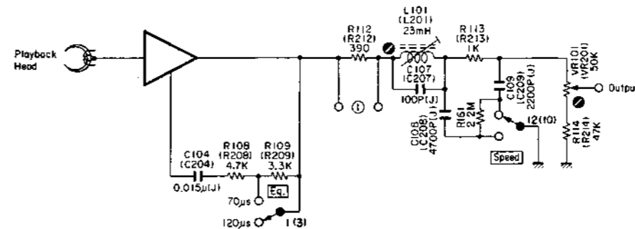
Fig. 6.19 Playback Amp.
