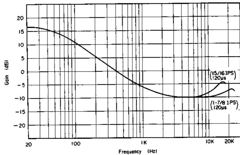
Fig. 6.21 Typical Playback Equalization Curve (1-7/8 / 15/16 ips)
