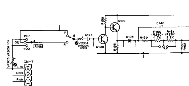
Fig. 6.2.12 19. Monitor Amplifier
