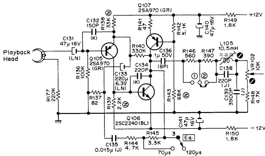
Fig. 2.2.1 Playback Eq. Amp. Circuit
