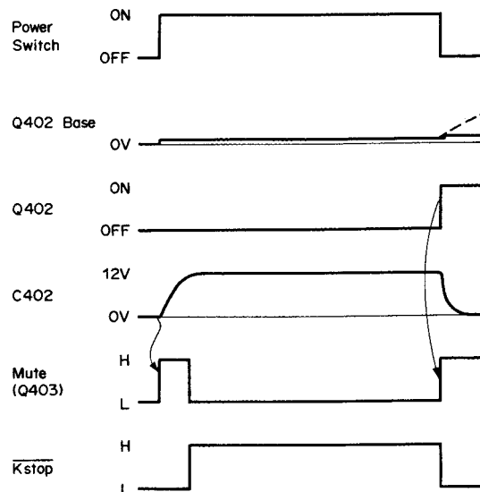
Fig. 2.3.14 Timing Chart
