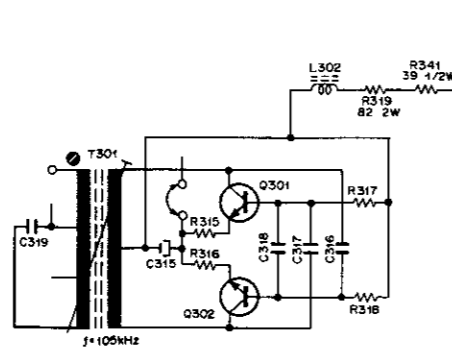
Fig. 6.2.9 11. Bias Oscillation Frequency and Erase Current
