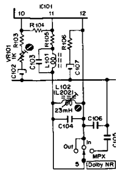
Fig. 6.2.7 5. MPX Filter
