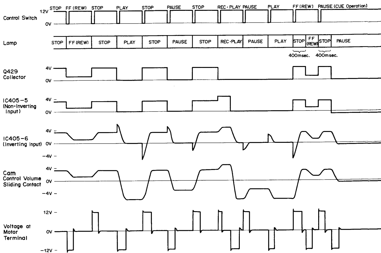
Fig. 2.3.23 Timing Chart
