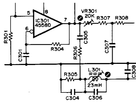
Fig. 6.2.3 2. Tone Calibration
