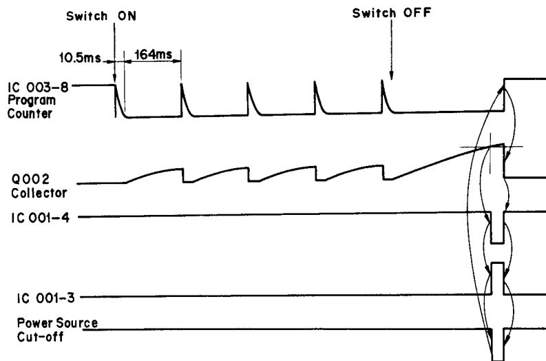
Fig. 2.4.5 Timing Chart
