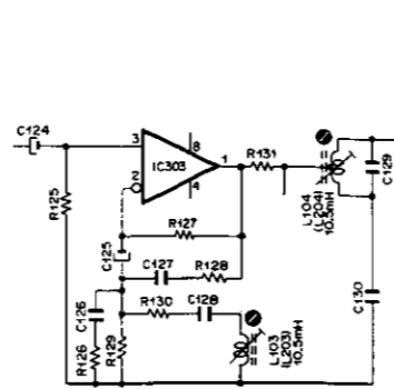
Fig. 6.1.9 11. Record Amplifier Equalizer 12. Bias Trap (Record Amp.) 17. Record/Playback Frequency Response
