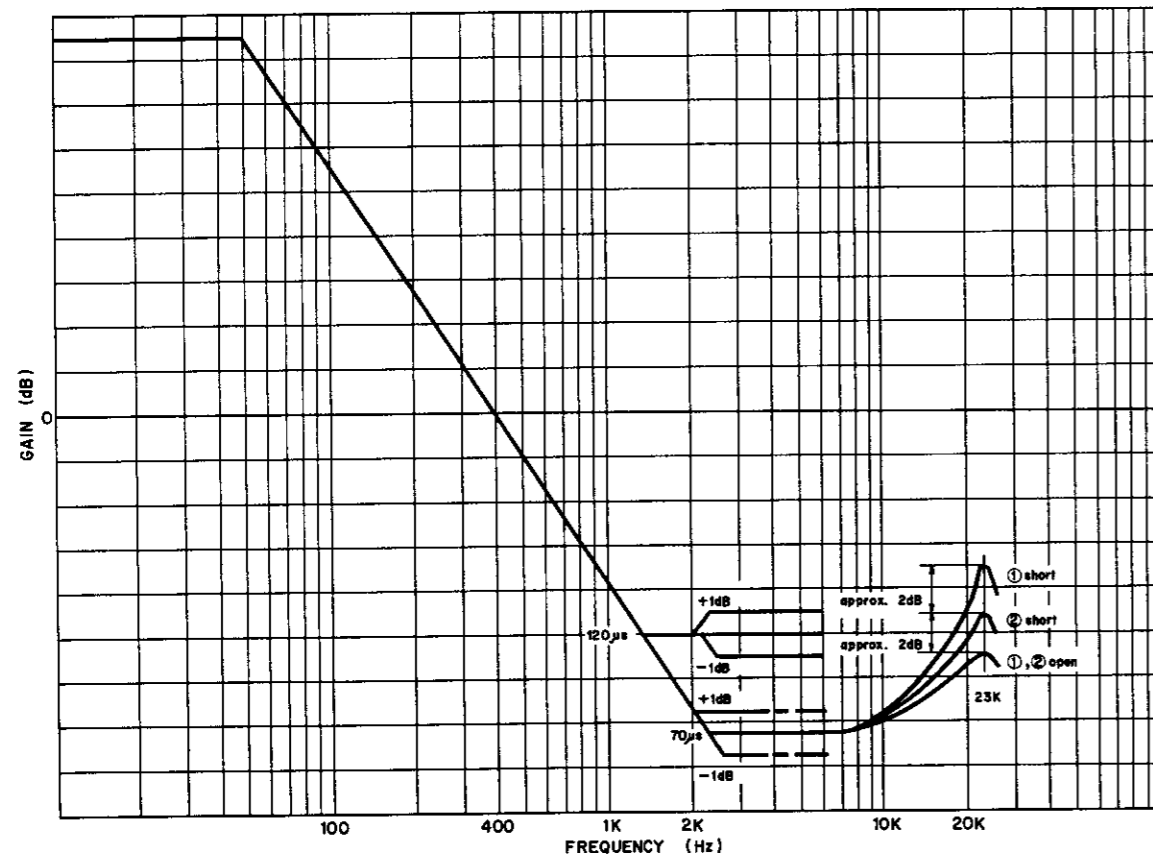
Fig. 6.1.12 Playback Equalization Curve
