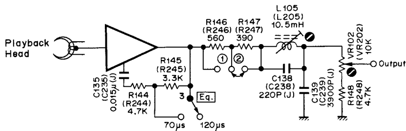
Fig. 2.2.2 System Diagram
