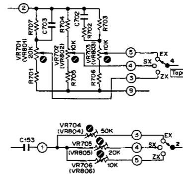
Fig. 6.1.10 16. Record Level and Recording Bias Current
