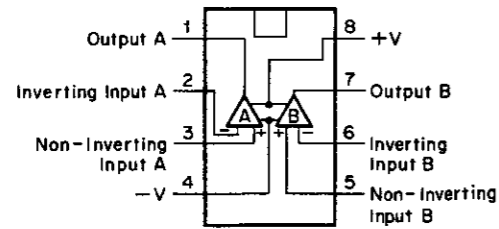
Fig. 13.4 Operational Amp. IC 4558
