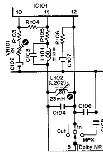
Fig. 6.1.4 2. Tone Calibration
