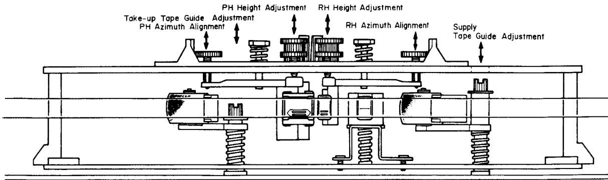
Fig. 2.1.6 Headblock
