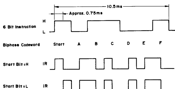
Fig. 2.4.2 Information Unit
