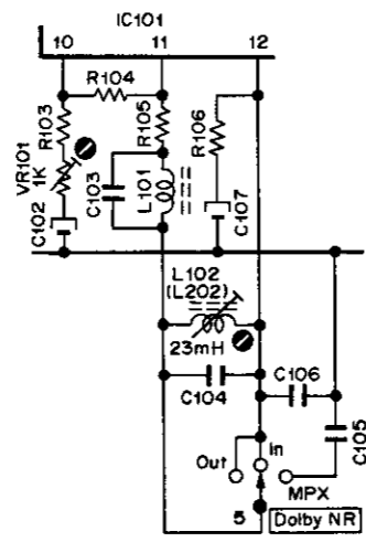
Fig. 6.2.4 2. Tone Calibration
