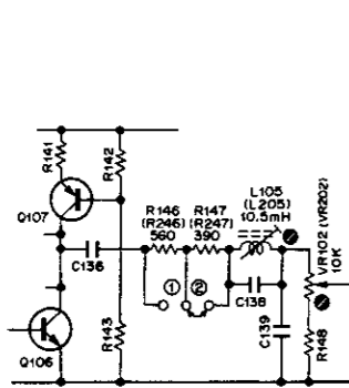
Fig. 6.1.7 7. Playback Level 13. Bias Trap (Playback Amp.)
