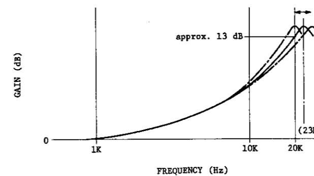
Fig. 6.1.14. Recording Peaking Curve
