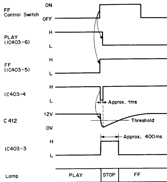
Fig. 2.3.16 Timing Chart
