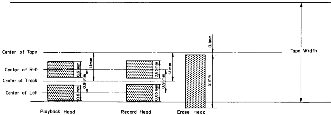
Fig. 2.1.7 Trackings
