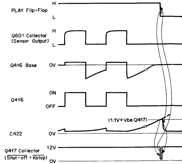
Fig. 2.3.21 Timing Chart
