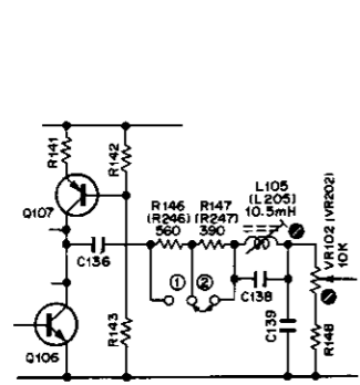
Fig. 6.2.8 8. Playback Level 14. Bias Trap (Playback Amp.)
