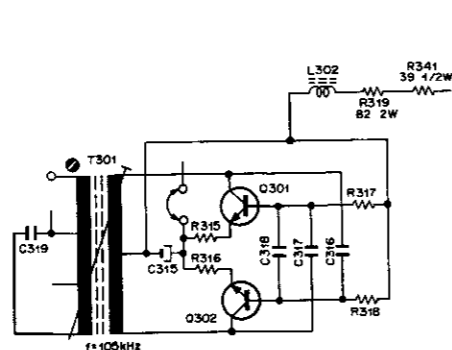
Fig. 6.1.8 10. Bias Oscillation Frequency and Erase Current
