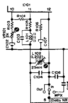
Fig. 6.1.6 4. MPX Filter
