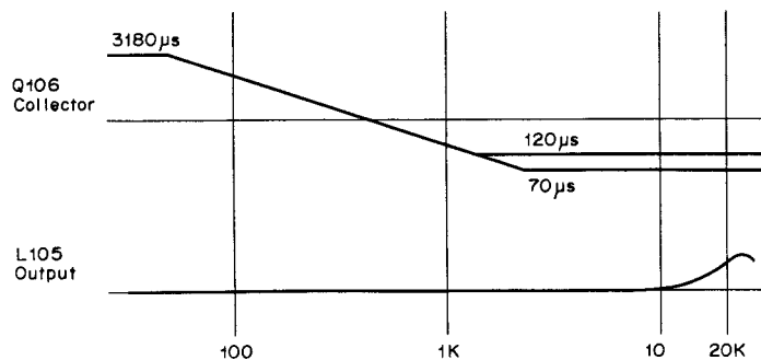
Fig. 2.2.3 Time Constant
