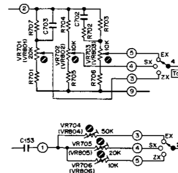
Fig. 6.2.11 17. Record Level and Recording Bias Current
