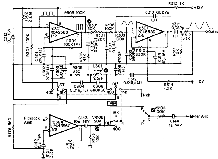
Fig. 2.2.6-A Test Tone Circuit
