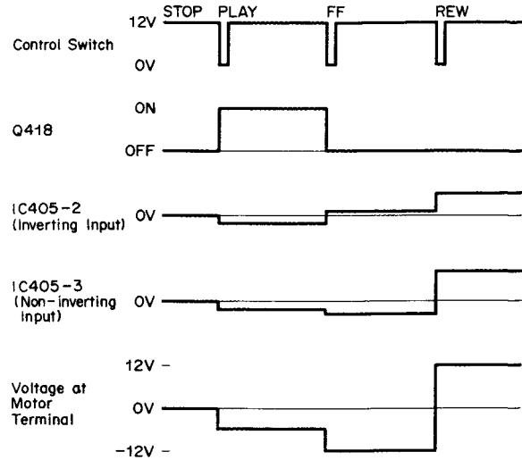
Fig. 2.3.25 Timing Chart
