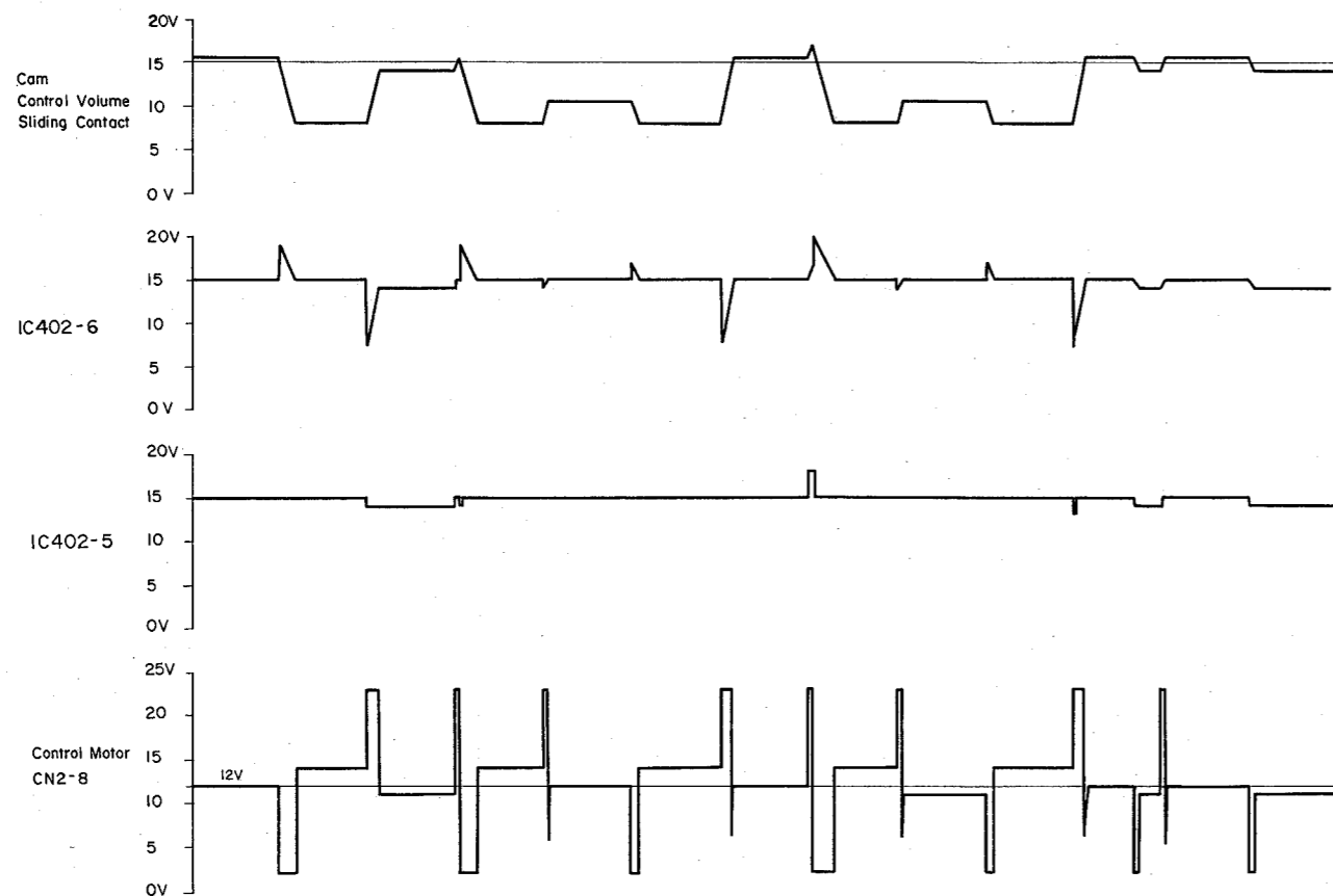
Fig. 2.3.11 Timing Chart
