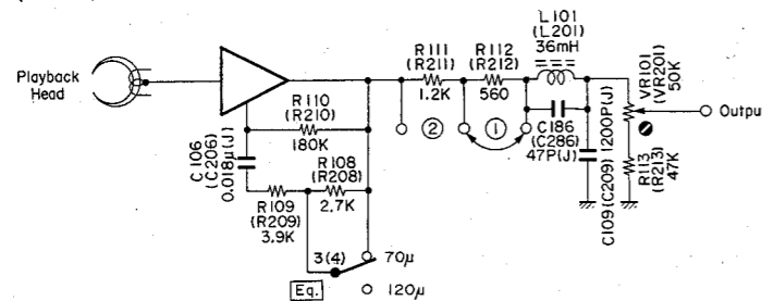
Fig. 7.8 Playback Amp.
