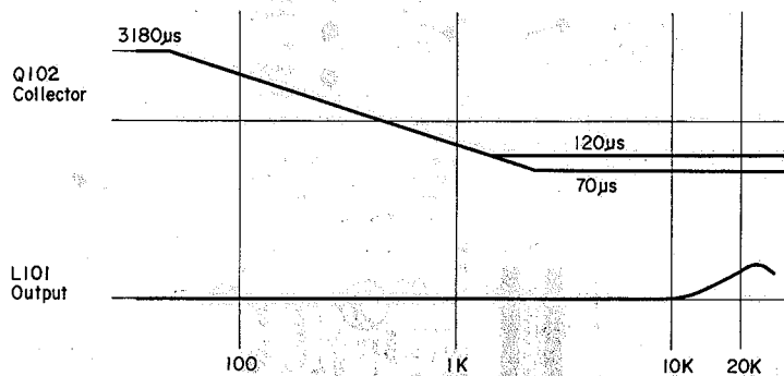
Fig. 2.2.3 Time Constant
