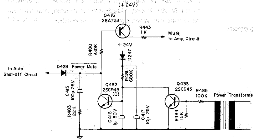
Fig. 2.3.3 Power-mute Circuit
