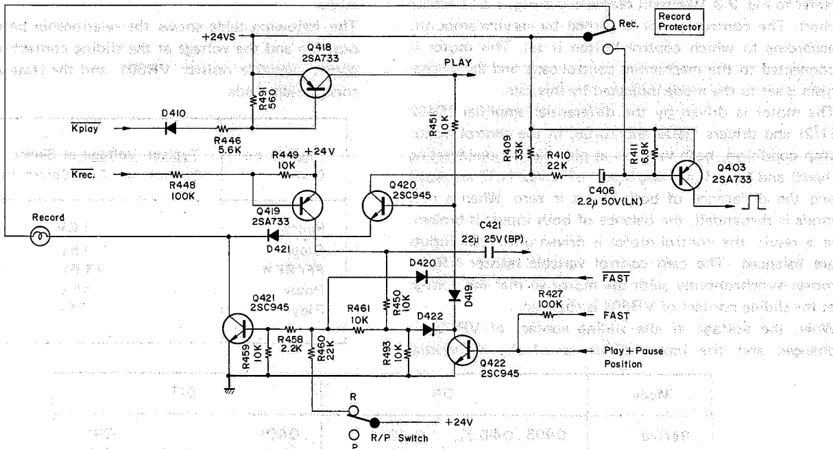
Fig. 2.3.8 Record Control Circuit
