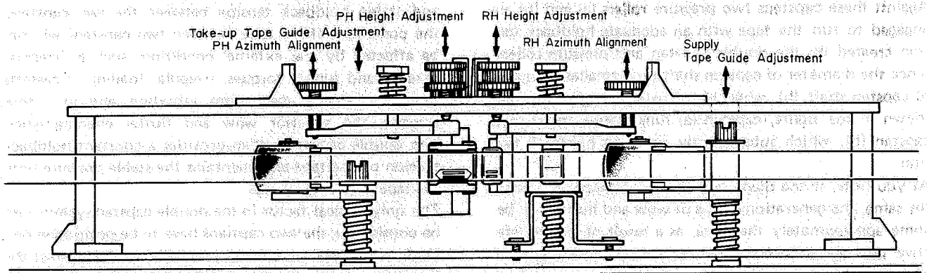
Fig. 2.1.1 Headblock
