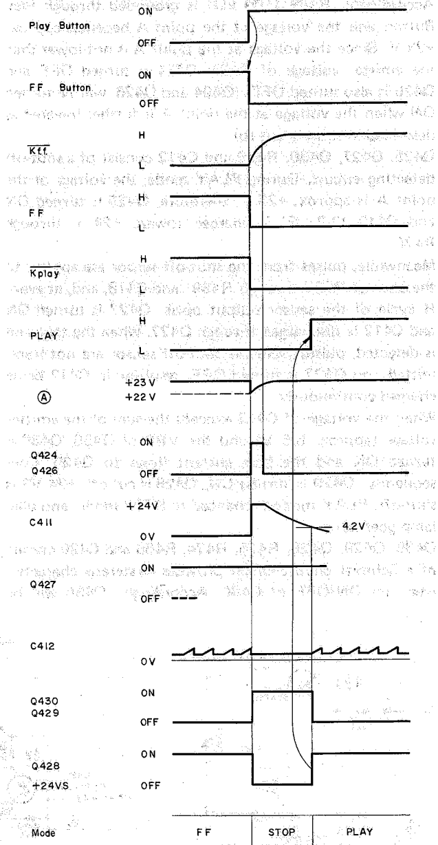
Fig. 2.3.7 Timing Chart
