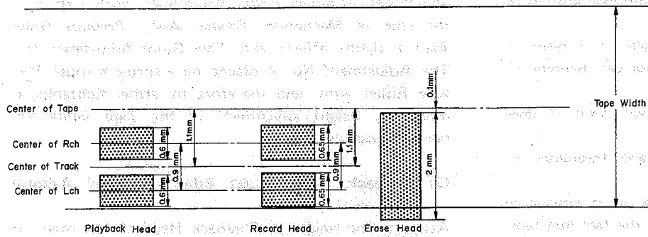
Fig. 2.1.2 Trackings
