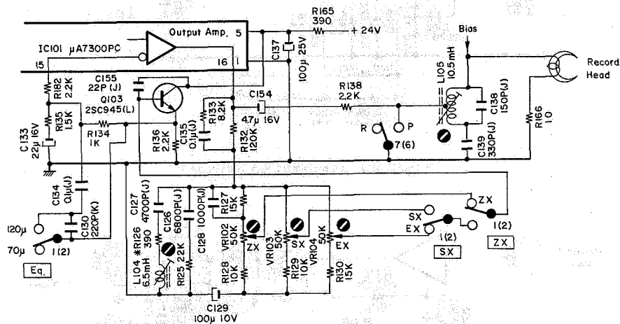
Fig. 2.2.4 Record Eq. Amp. Circuit
