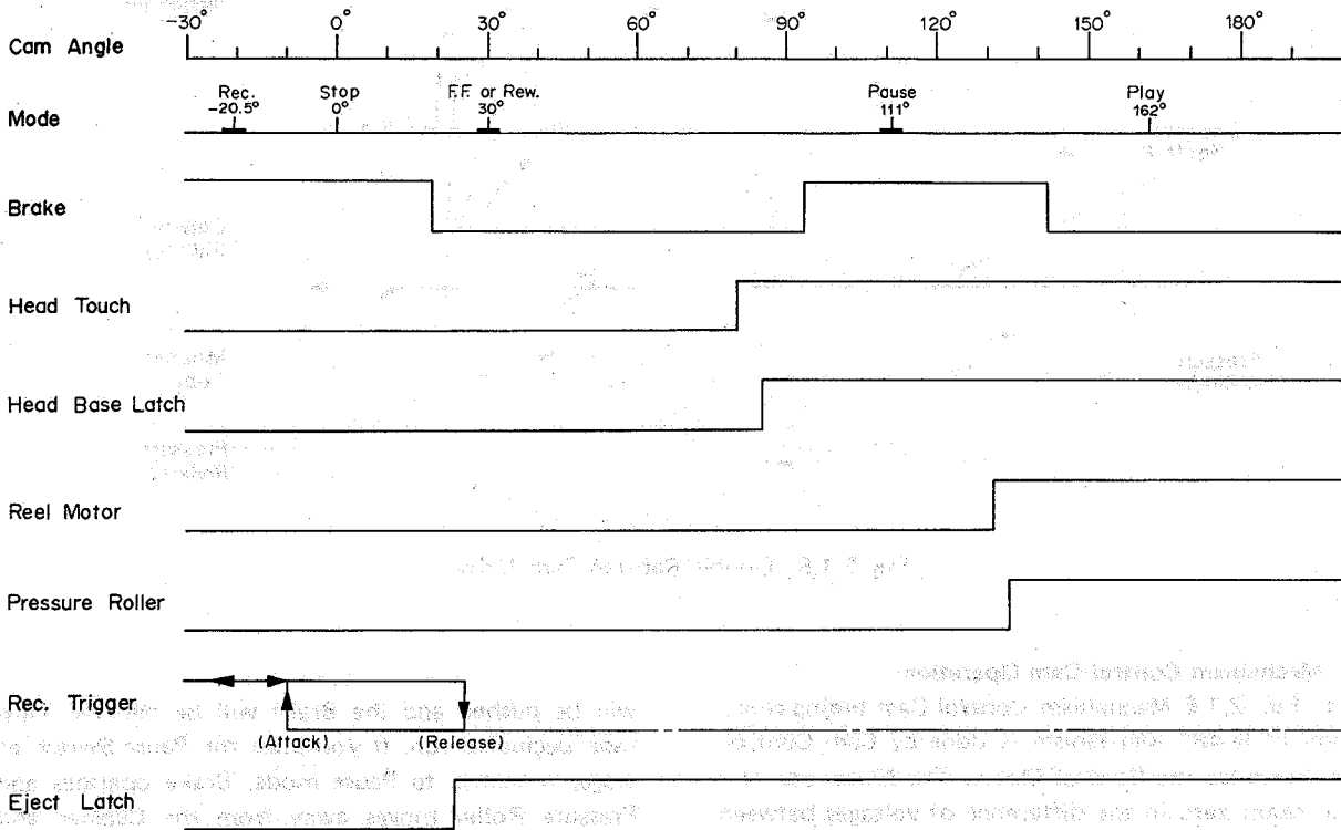
Fig. 2.1.6 Mechanism Control Cam Timing Chart
