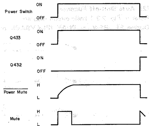
Fig. 2.3.4 Timing Chart
