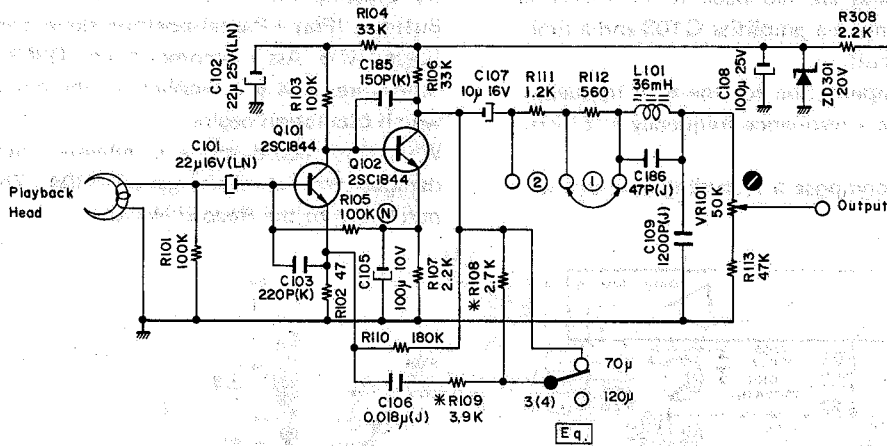
Fig. 2.2.1 Playback Eq. Circuit
