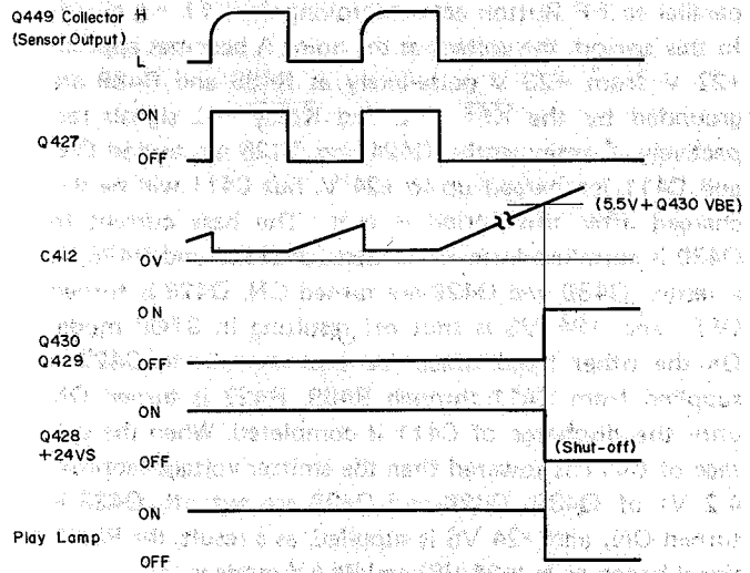
Fig. 2.3.6 Timing Chart
