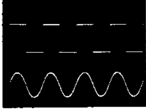
IC702 ④ pin Capstan frequency generator pulse (output) 2V/Division 0.5msec/Division Connector AW ③ pin Capstan frequency generator signal (input) 1V/Division 0.5msec/Division —Record mode—
