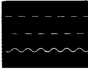
IC702 ②③ pin Drum frequency generator pulse (output) 2V/Division 1msec/Division Connector AN ③ pin Drum frequency generator signal (input) 50mV/Division 1msec/Division —Record mode—
