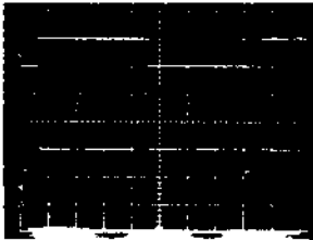
IC701 ⑧ pin Head switching pulse 5V/Division 5msec/Division IC701 ⑥ pin Drum pulse generator MM 2V/Division 5msec/Division IC701 ⑦ pin Drum pulse generator (input) 2V/Division 5msec/Division
