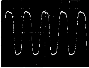
Y/C Module ⑩ pin 4.43 MHz oscillation signal 200mV/Division 0.1µsec/Division
