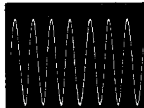
Connector BA ④, ⑤ pin (Between Audio erase head and Ground.) 10V/Division 10µsec/Division —Record mode—
