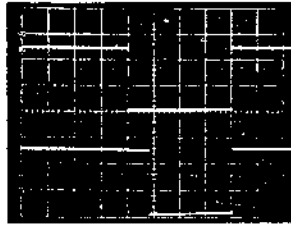
TP701 (1) pin Head switching pulse 2V/Division 5msec/Division TP701 (2) pin Tracking MM pulse 2V/Division 5msec/Division — Record mode —
