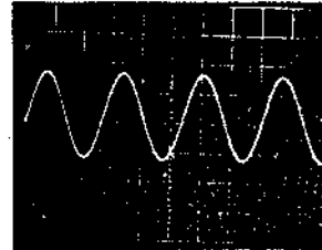
Socket AM (19) pin Capstan frequency generator signal 500mV/Division 0.5msec/Division
