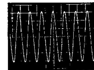
K602 (9), (11) pin (Between audio erase head and ground) 10V/Division 10μsec/Division — Record mode —
