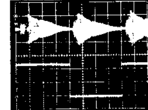
TP1 Playback preamp. signal 200mV/Division 5msec/Division TP2 Head switching pulse 2V/Division 5msec/Division — Playback mode — (Sweep tape)
