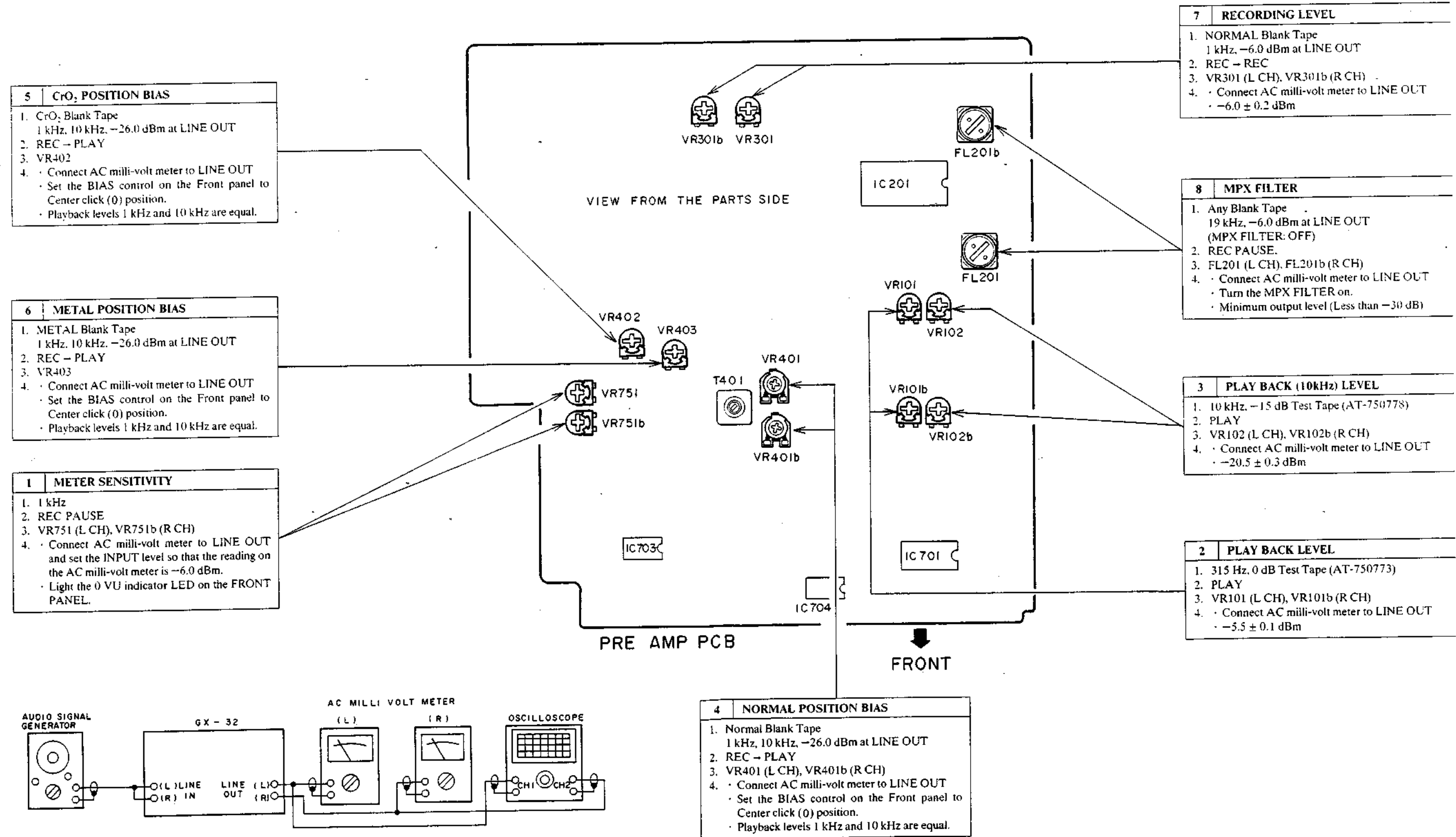
Fig. 5-1 INSTRUMENTS CONNECTION
