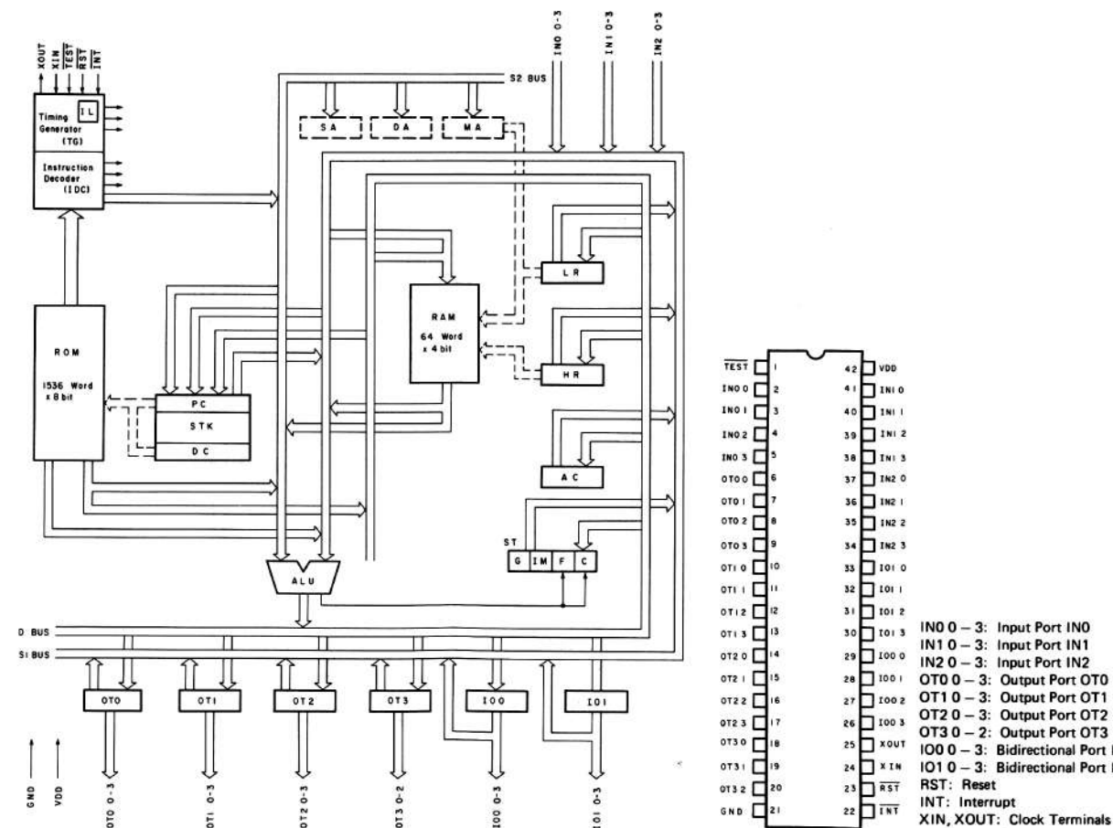
Fig. 8.1.7 4-Bit Micro-processing Unit TMP4315BP-1814
