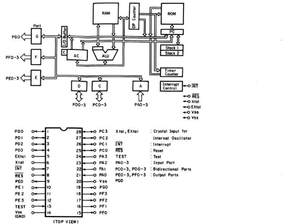
Fig. 8.1.6 4-Bit Micro-processing Unit LM6416E-106
